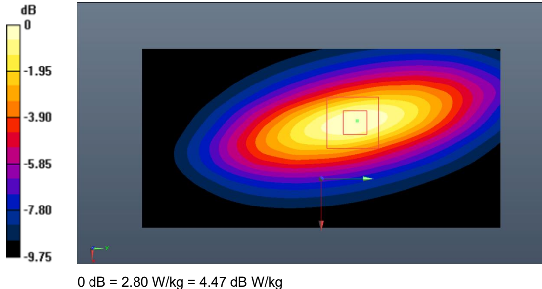
Fig.B.1. Validation 750MHz 250mW
