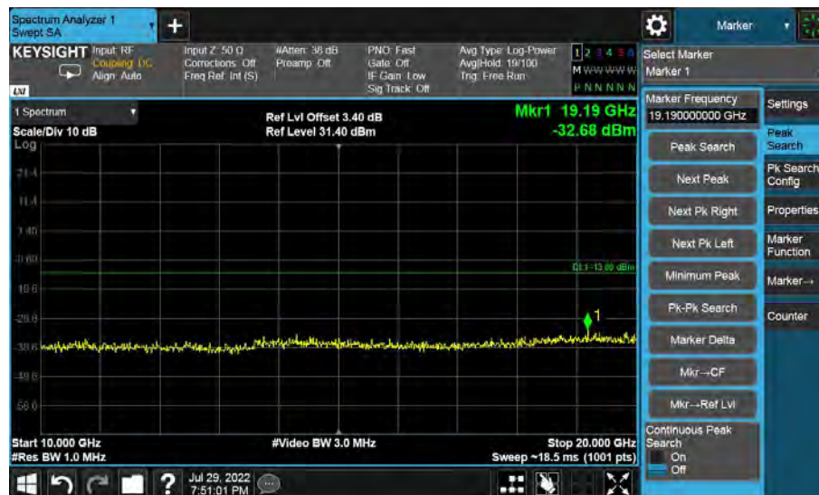
10GHz to 20GHz, Low Channel, Subcarrier (15kHz), QPSK, 12@0
