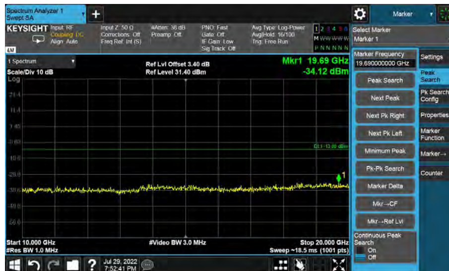
10GHz to 20GHz, Low Channel, Subcarrier (15kHz), BPSK, 1@0
