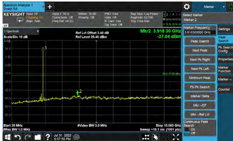
30MHz to 10GHz, Mid Channel, Subcarrier (3.75kHz), QPSK, 1@0
