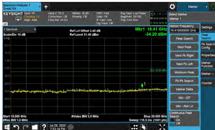
10GHz to 20GHz, Low Channel, Subcarrier (15kHz), QPSK, 1@0
