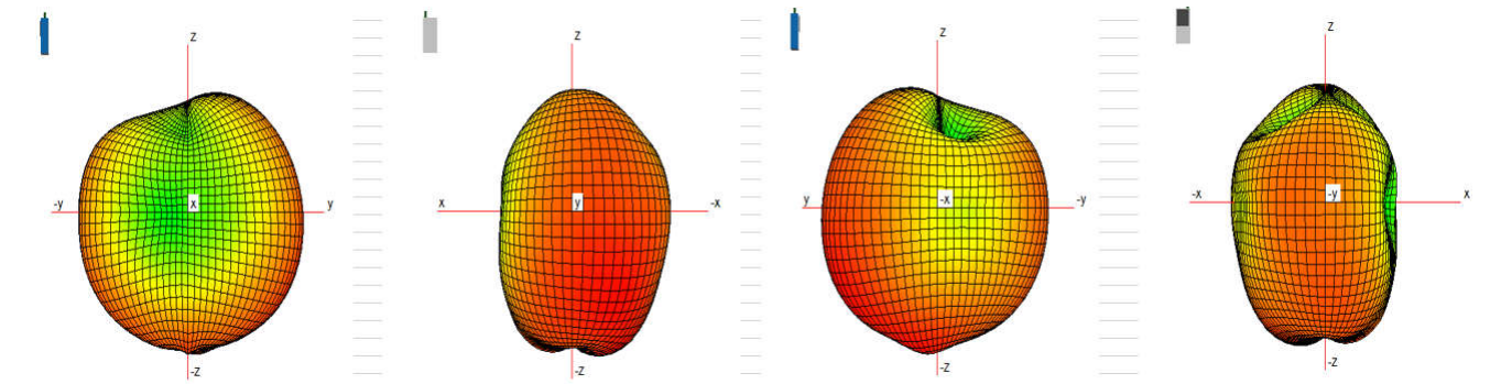
GSM900/WCDMA B8
