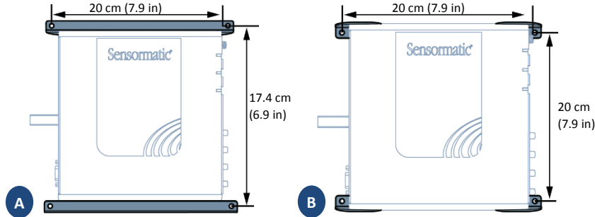
Figure 3. Mounting bracket orientations
