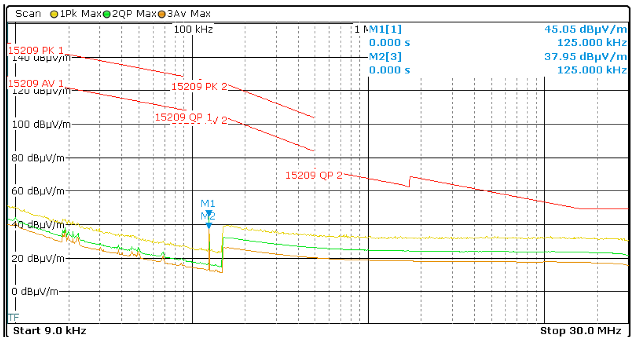
Figure 8: Chart of radiated emissions test below 30 MHz, EUT position Y, antenna polarization in line, without tag
