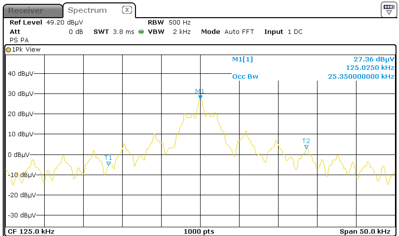
Figure 7: Chart of occupied bandwidth test, with tag
