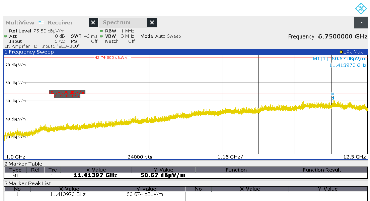
Figure 10: Chart of radiated emissions pre-measurement from 1 GHz to 12.5 GHz, EUT position Y, with tag, antenna polarization horizontal
