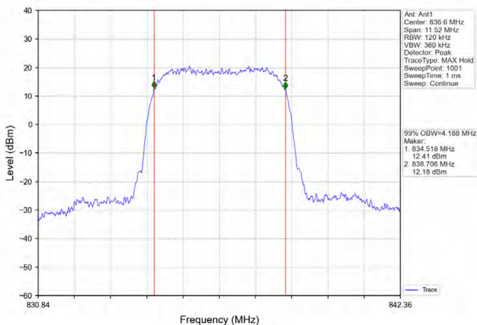
Band5_RMC_MCH_836.6MHz_12.2kbps RMC_NTNV
