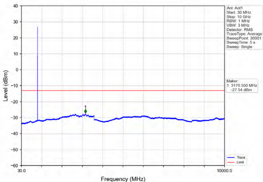
GSM850_GSM_LCH_824.2MHz_NTNV
