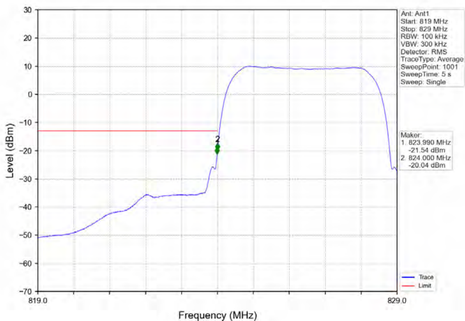
Band5_RMC_LCH_826.4MHz_12.2kbps RMC_NTNV
