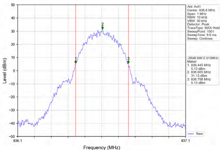
GSM850_GSM_MCH_836.6MHz_NTNV
