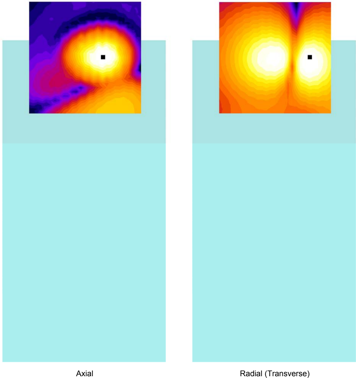
Figure 9-1 T-Coil Scan Overlay Magnetic Field Distributions
