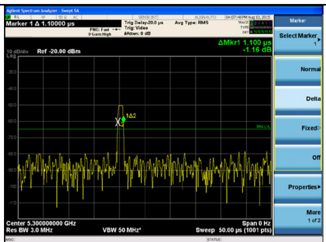
Radar Calibration - Type 0 (Single Burst)
