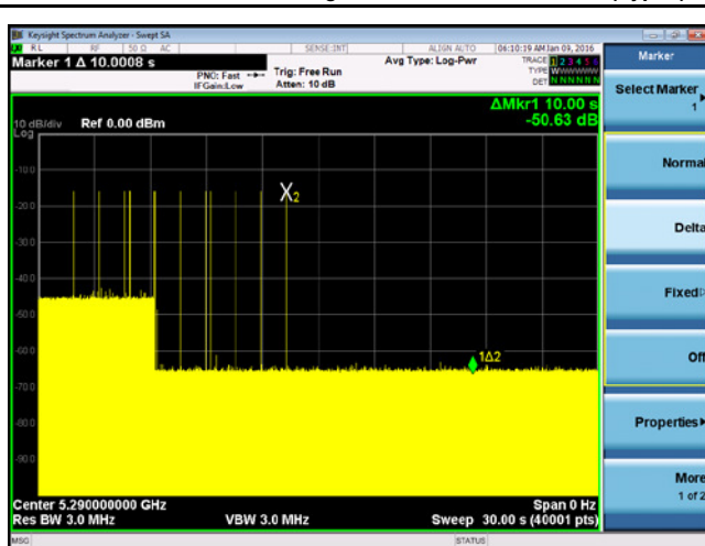
Channel Move Time& Closing Time - 802.11ac-5290MHz (Type5)
