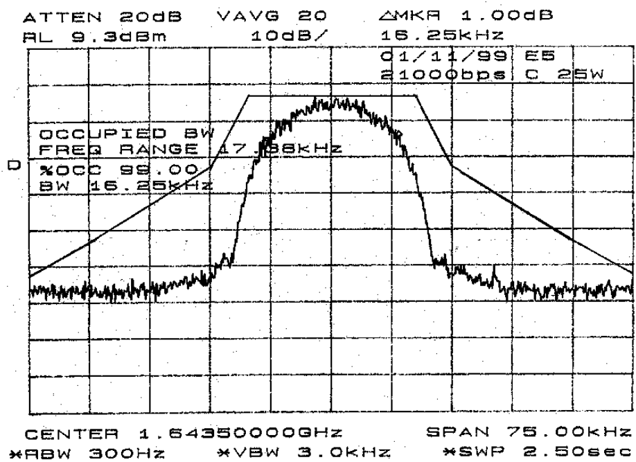
Figure 9.6.2.5 Bandwidth Occupancy Test – Power 25 Watts
