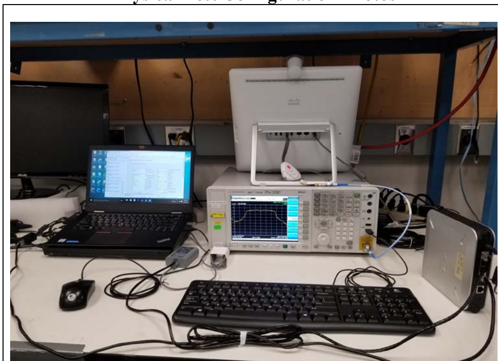
Title: RF Conducted Emissions Test Set Up
