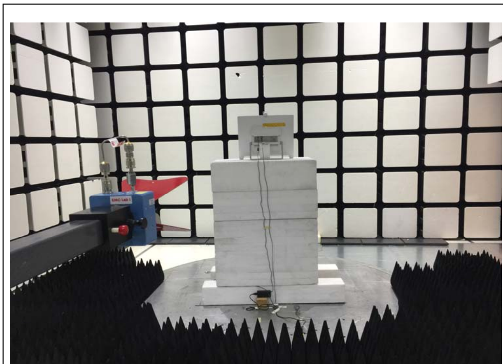
Title: Radiated Emissions 1 – 18 GHz Test Set Up
