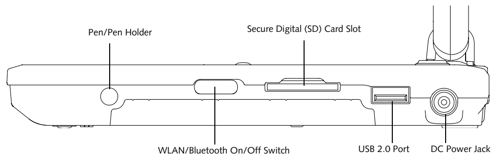
Figure 2-6. LifeBook P Series notebook/Tablet PC right-side panel
