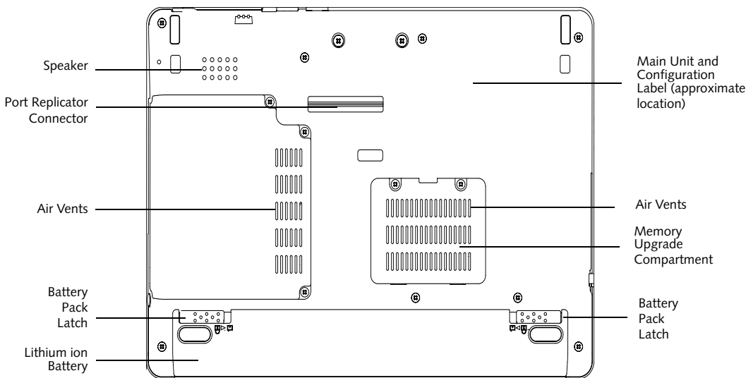
Figure 2-8. LifeBook P Series notebook/Tablet PC bottom panel
