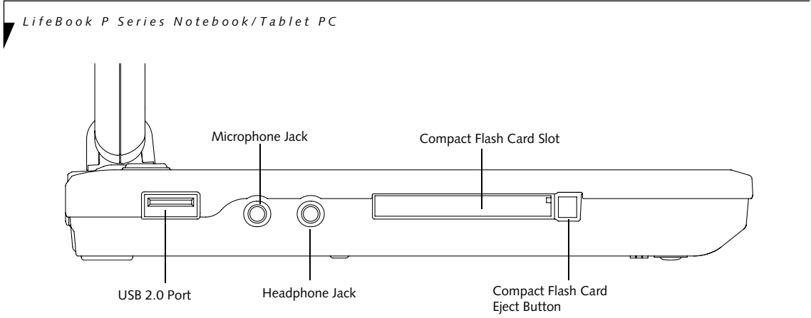
Figure 2-5. LifeBook P Series notebook/Tablet PC left-side panel
