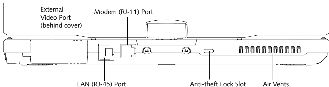
Figure 2-7. LifeBook P Series notebook/Tablet PC rear panel
