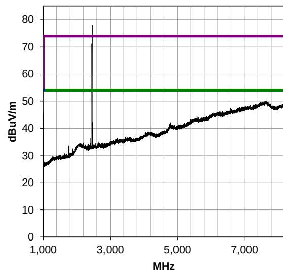
1000-8200 MHz, Run 2
