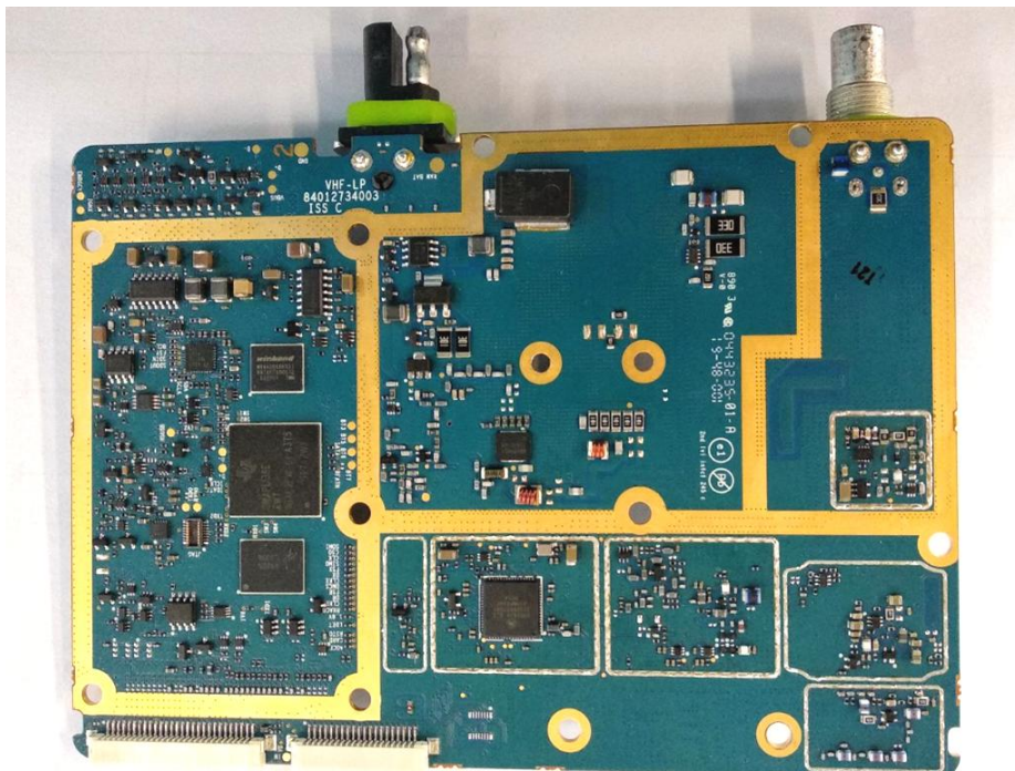
RF board without Shields (Bottom)
