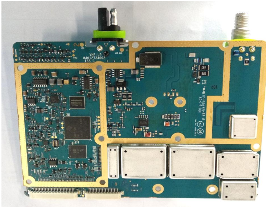
RF board with Shields (Bottom)
