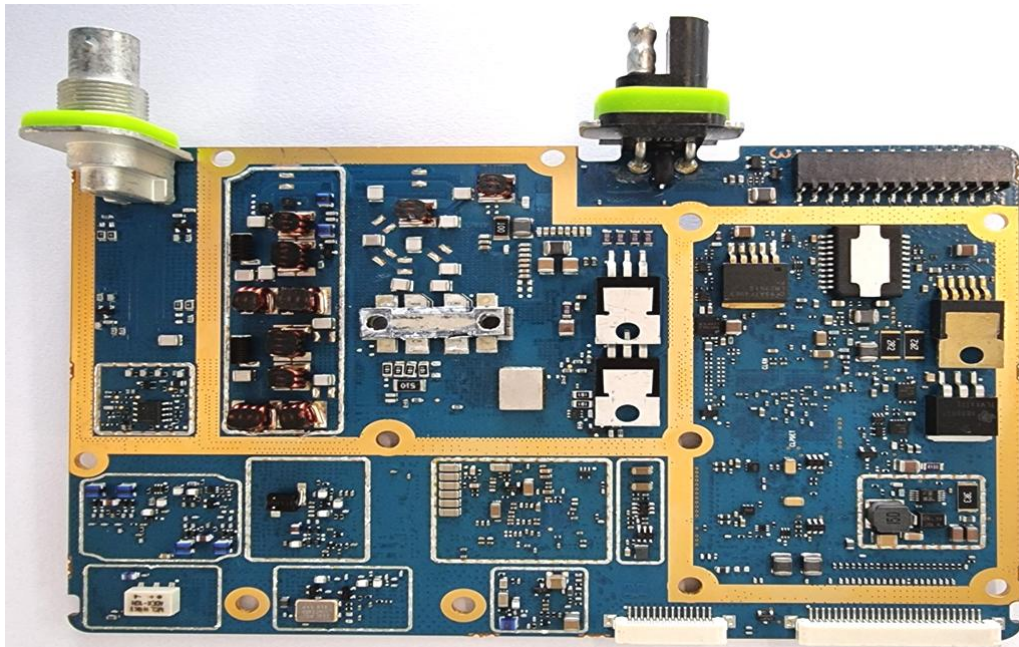
RF board without Shields (Top)
