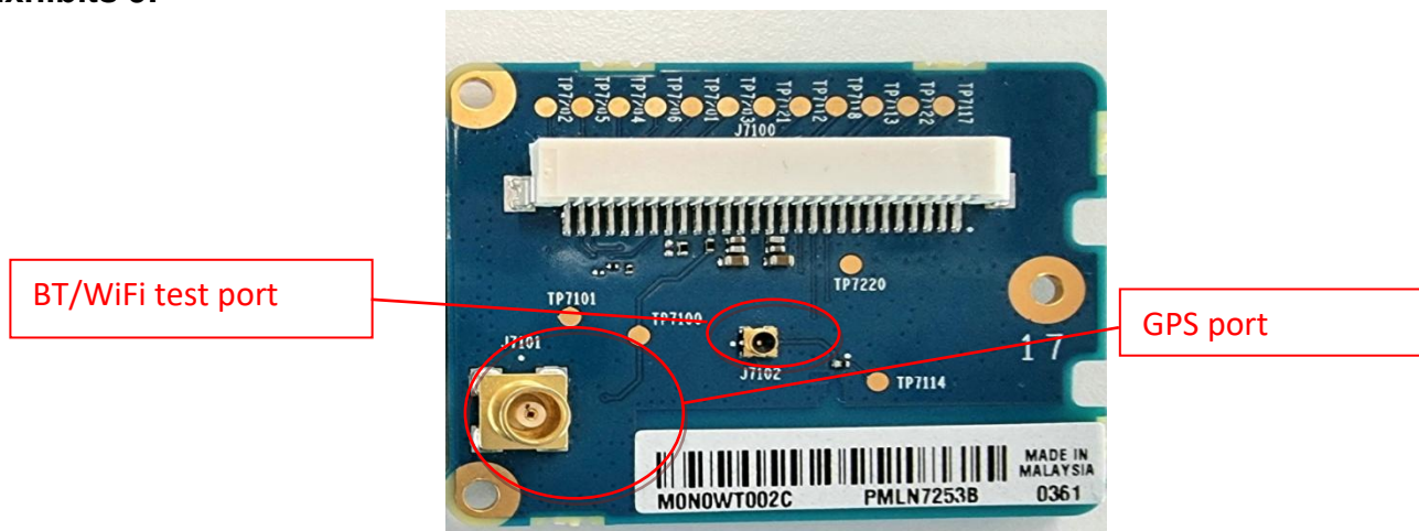
Expansion board (Top)
