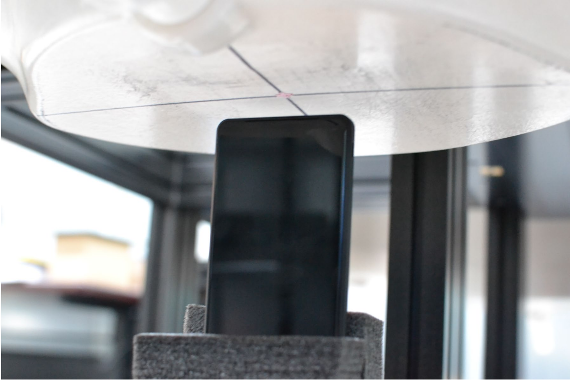
SAR Test Setup Photo 11 – Hotspot, Bottom Edge, 10 mm
