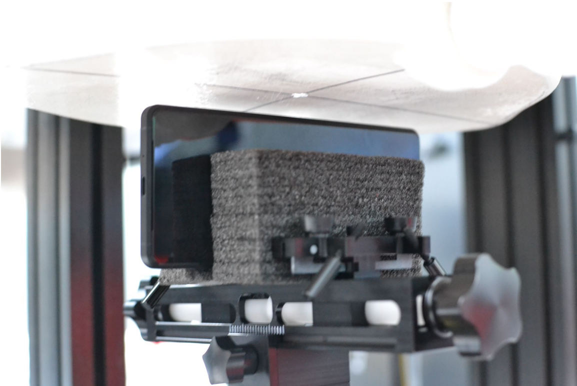
SAR Test Setup Photo 14 – Hotspot, Left Edge, 10 mm
