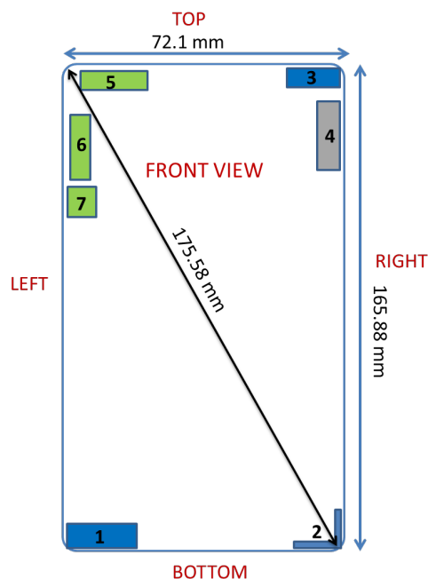
Figure E-1 DUT Antenna Locations
