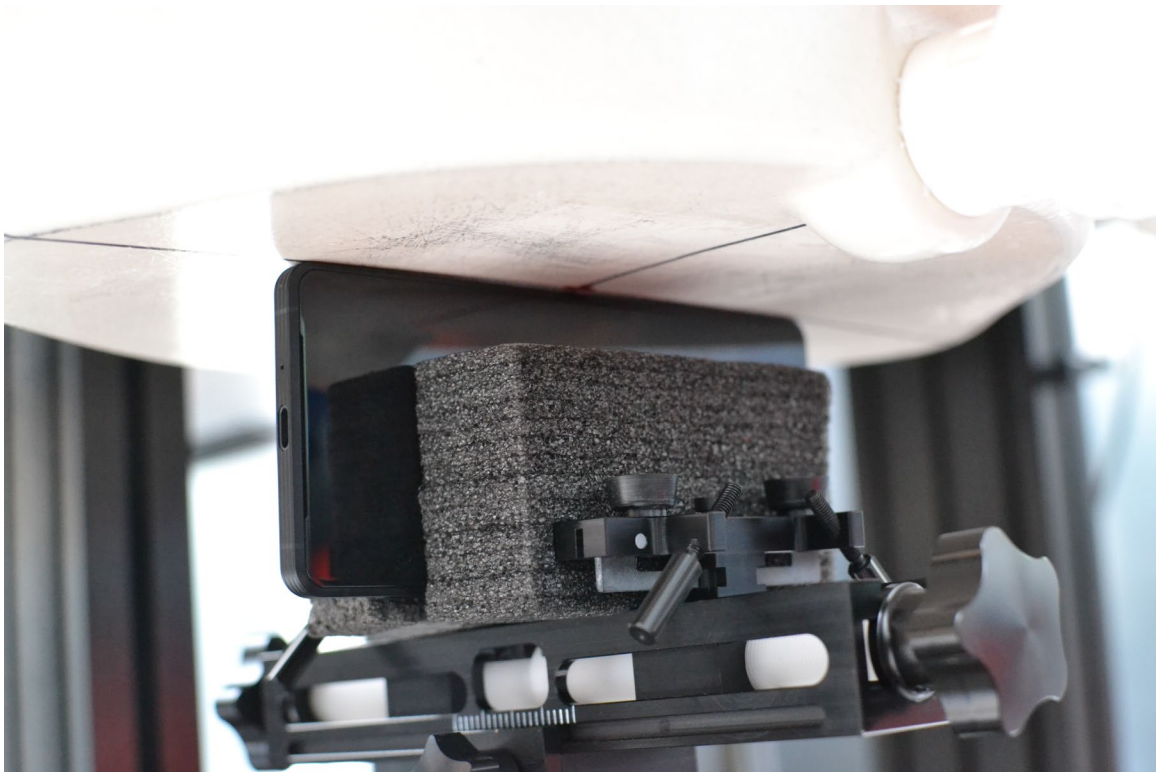
SAR Test Setup Photo 15 – Phablet, Left Edge, 0 mm
