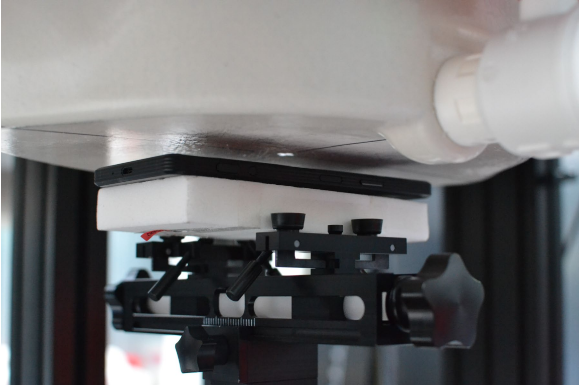
SAR Test Setup Photo 7 – Hotspot, Front Side at 10 mm
