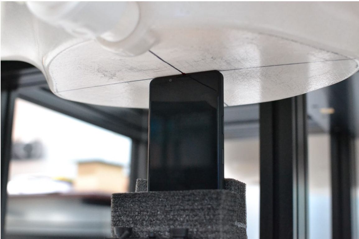
SAR Test Setup Photo 10 – Phablet, Top Edge, 0 mm
