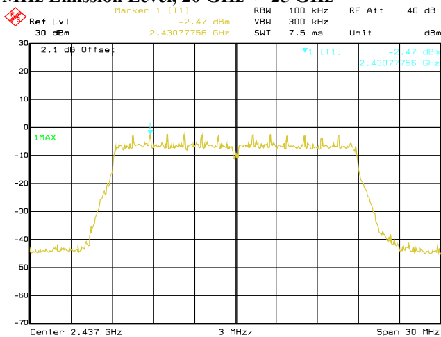
Conducted Emissions. 802.11n, Frequency 2437 MHz Reference Level
