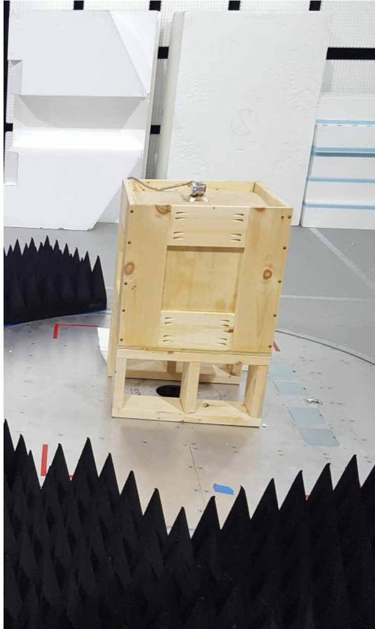
RADIATED FRONT PHOTO
