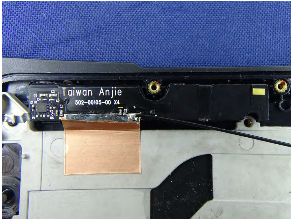
(101) EUT Phot – WWAN Main Antenna
