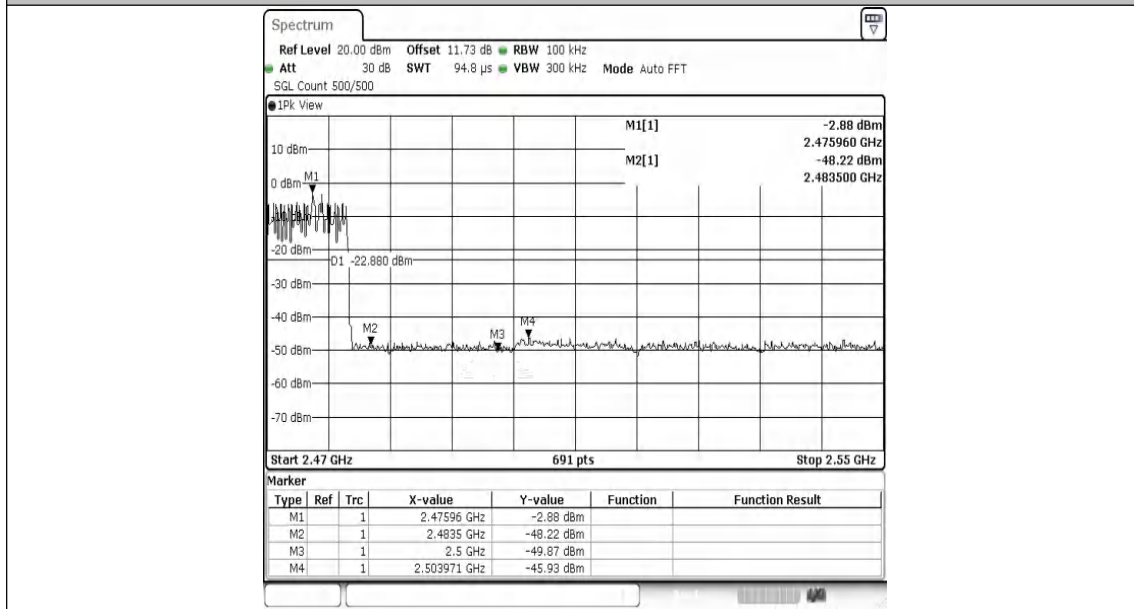
3DH5-Ant1-Hop_2480-PASS
