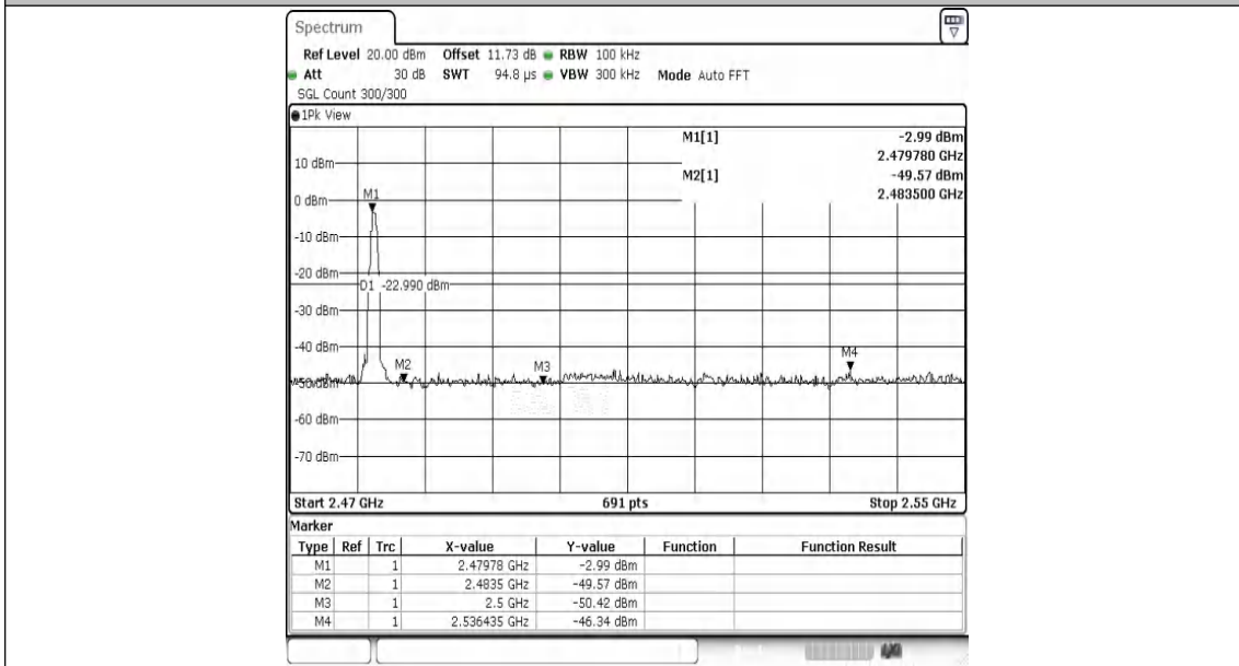
2DH5-Ant1-2480-PASS
