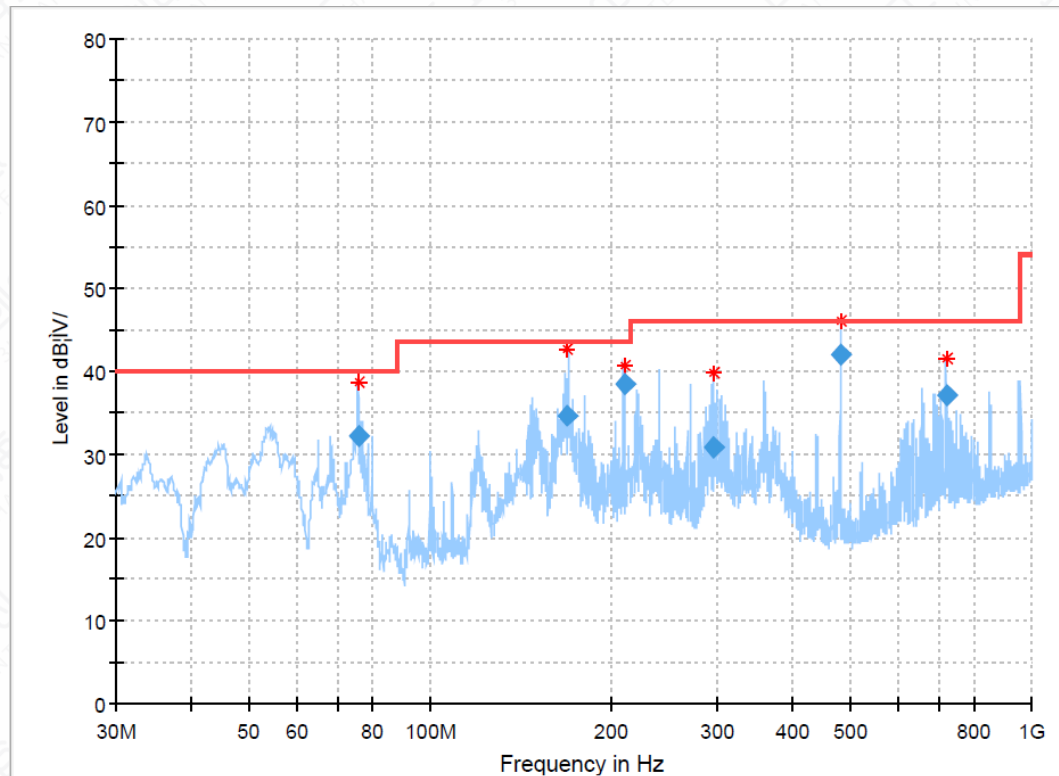
Figure A.1-1 Mode 2 (30M-1GHz) _ S02aa (Mainly Supply)
