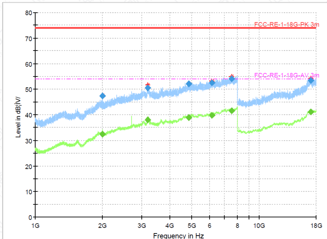
Figure A.1-6 Mode 1 (1GHz-18GHz)-V _ S11aa (Secondary Supply)
