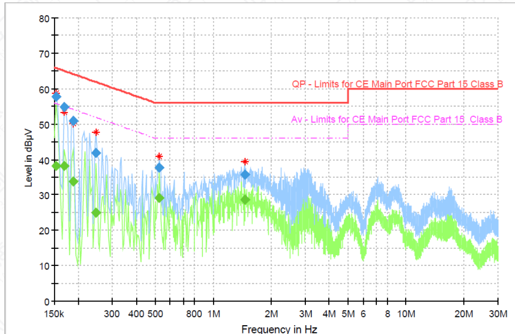
Figure A.2-1 Mode 1 (150kHz-30MHz) _ S02aa (Mainly Supply)
