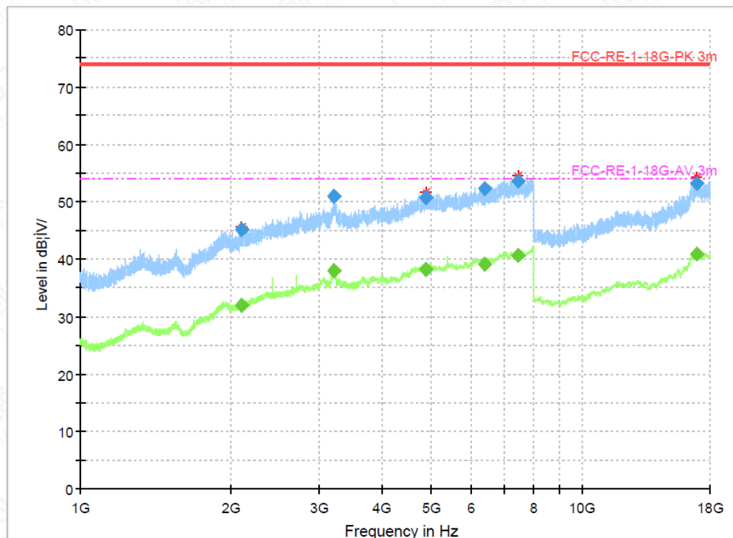
Figure A.1-2 Mode 2 (1GHz-18GHz)-H _ S02aa (Mainly Supply)
