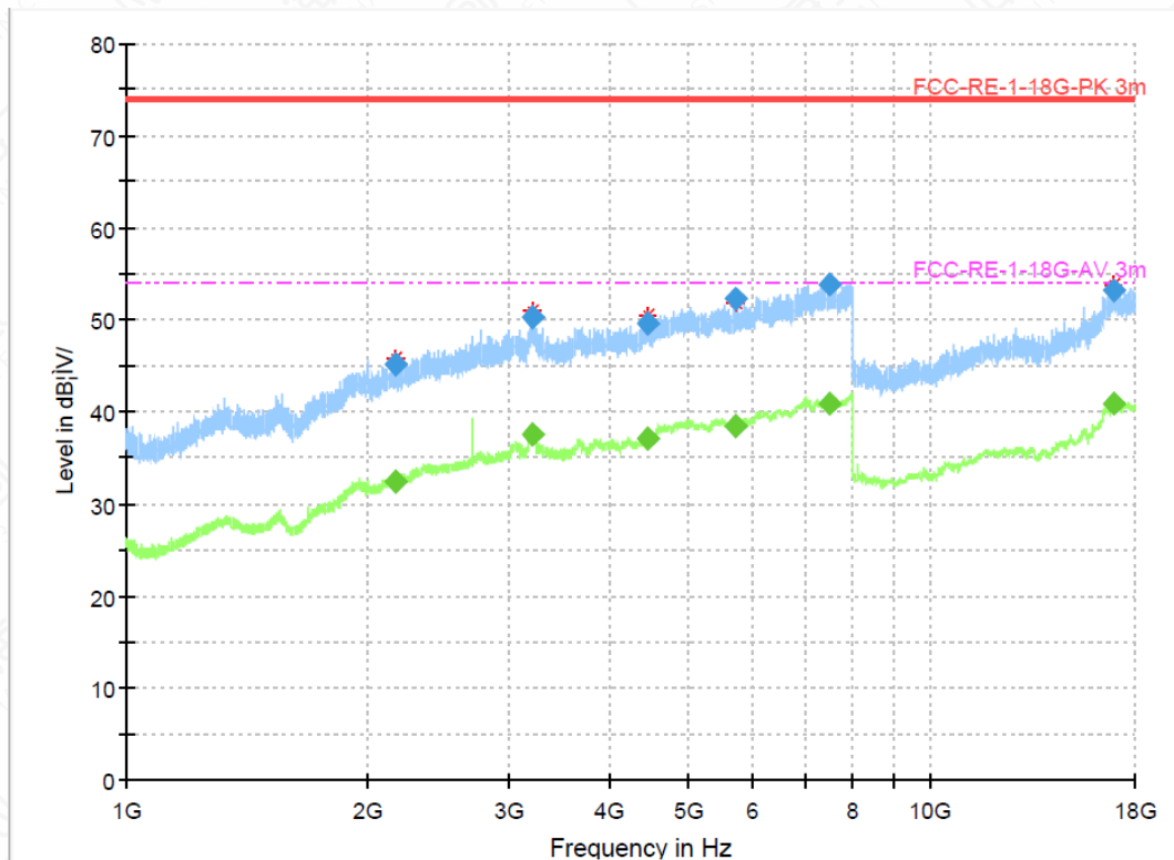
Figure A.1-3 Mode 2 (1GHz-18GHz)-V _ S02aa (Mainly Supply)
