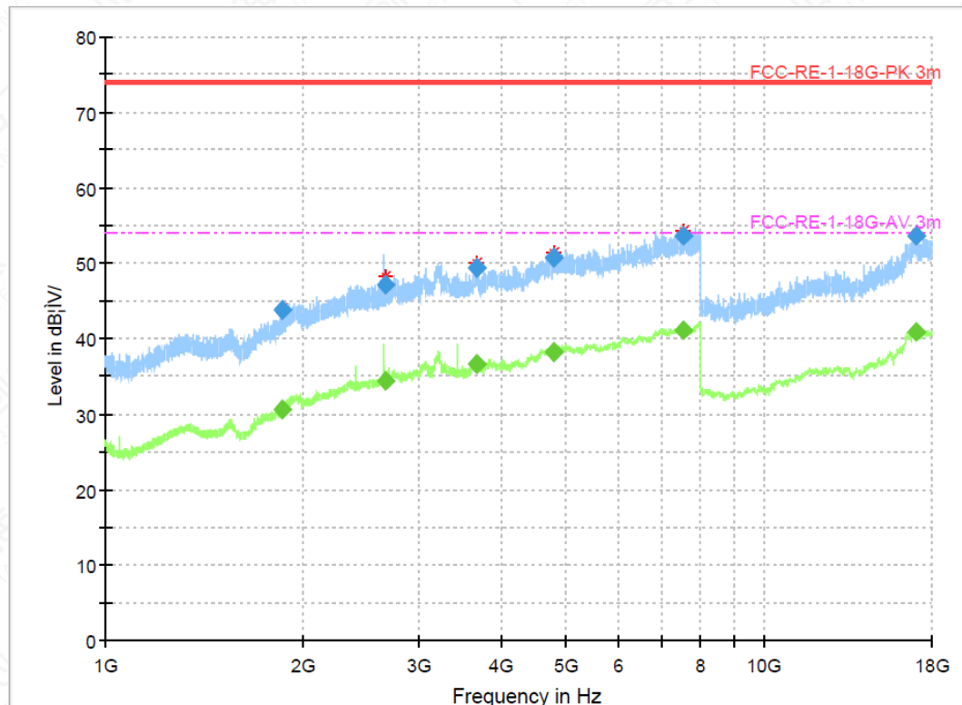
Figure A.1-5 Mode 1 (1GHz-18GHz)-H _ S11aa (Secondary Supply)
