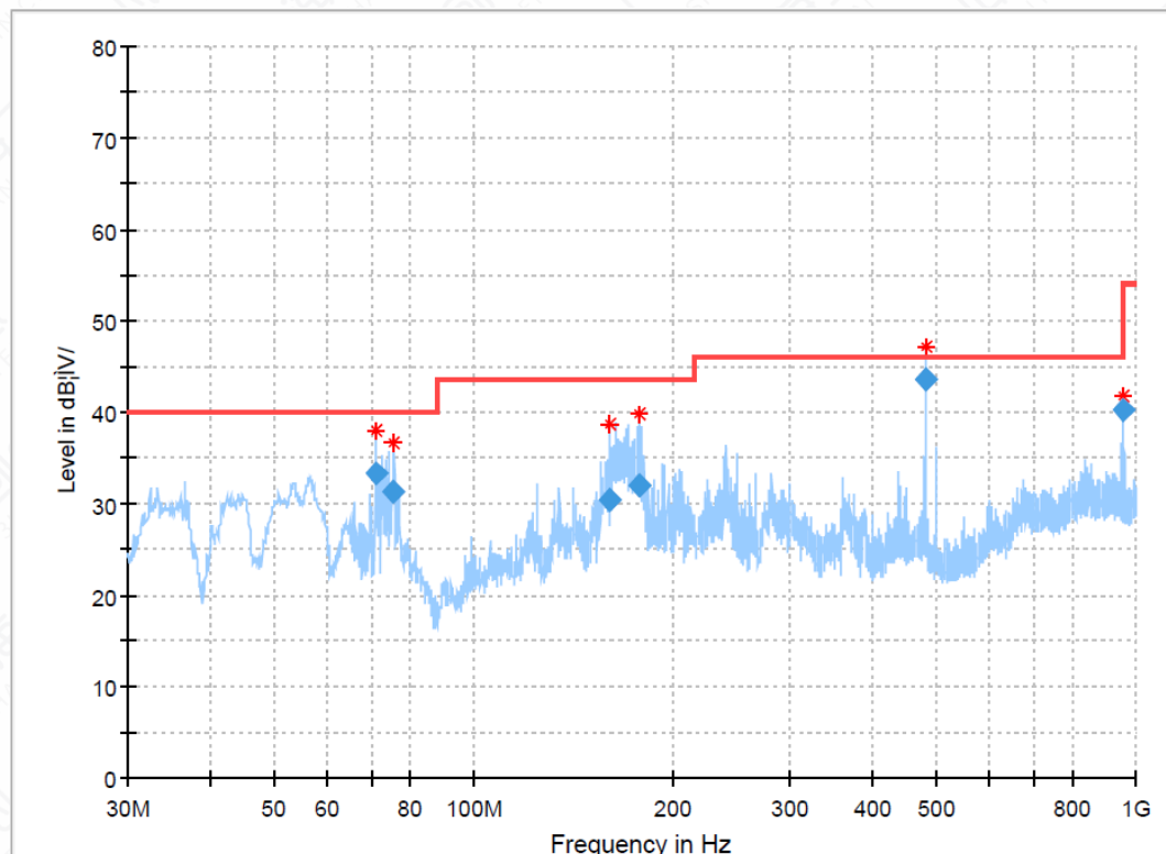
Figure A.1-4 Mode 1 (30M-1GHz) _ S11aa (Secondary Supply)
