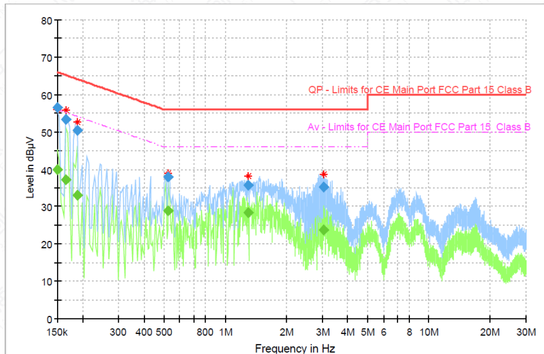
Figure A.2-2 Mode 1 (150kHz-30MHz) _ S11aa (Secondary Supply)
