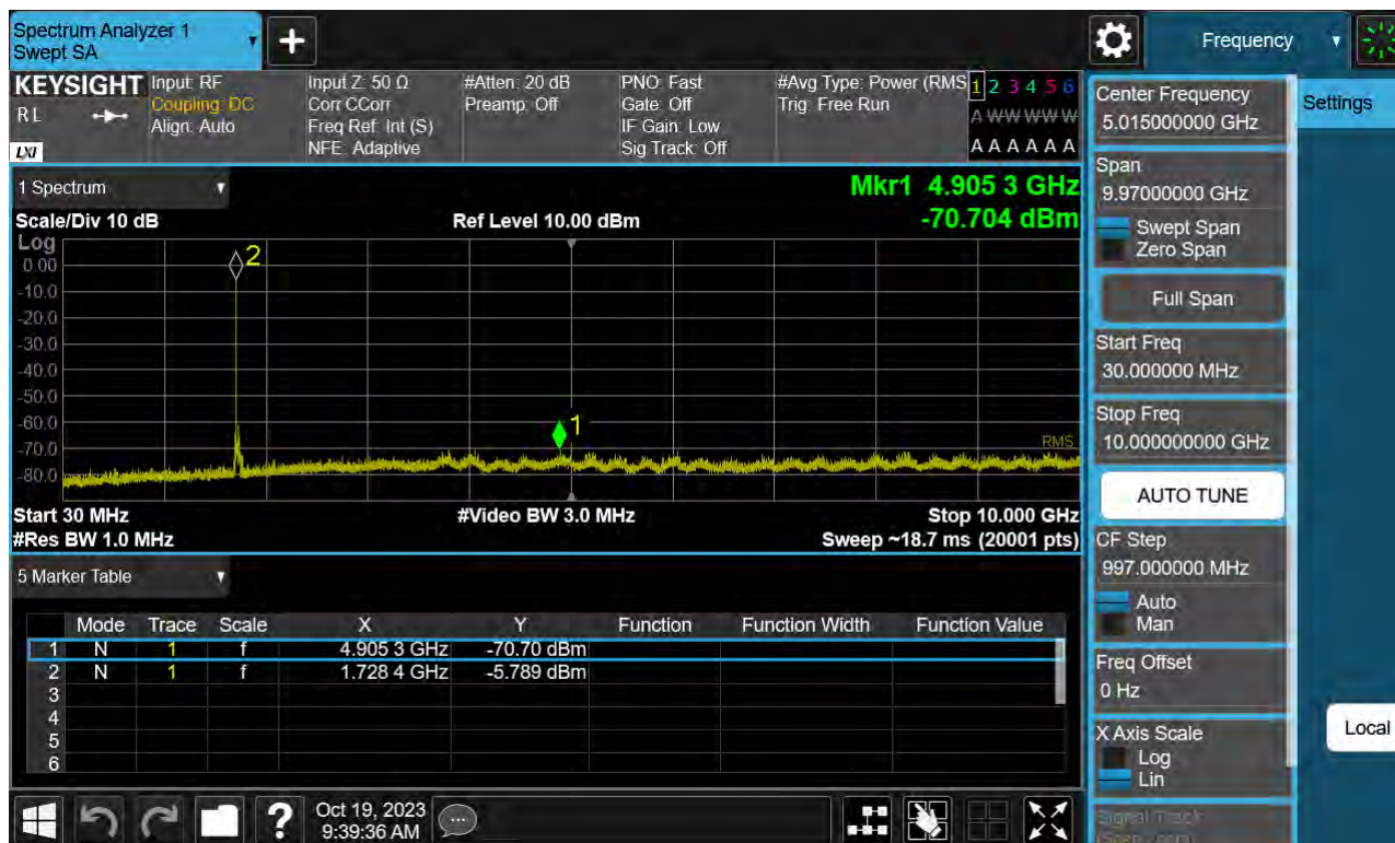
Sub6 n66. Conducted Spurious Plot_1 (349000ch_35 MHz_BPSK_ RB 1_1)
