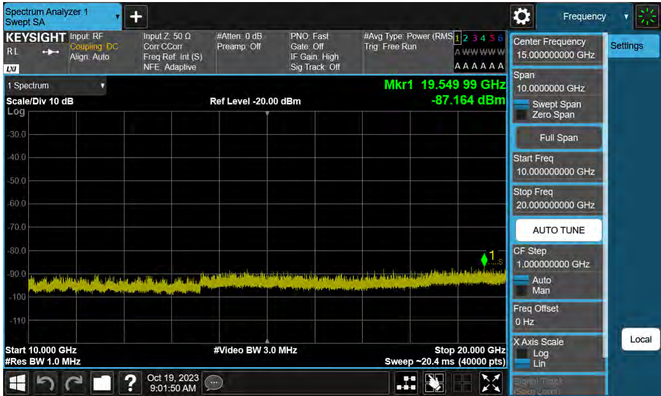
Sub6 n66. Conducted Spurious Plot_2 (353500ch_25 MHz_BPSK_ RB 1_1)
