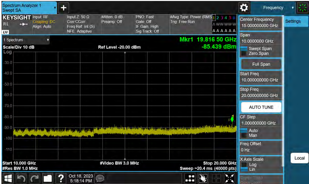
Sub6 n66. Conducted Spurious Plot_2 (344000ch_20 MHz_BPSK_ RB 1_1)
