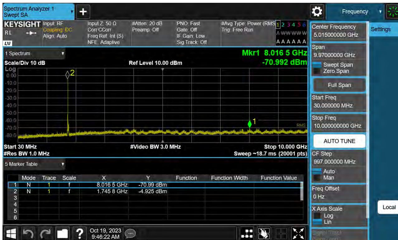
Sub6 n66. Conducted Spurious Plot_1 (352500ch_35 MHz_BPSK_ RB 1_1)
