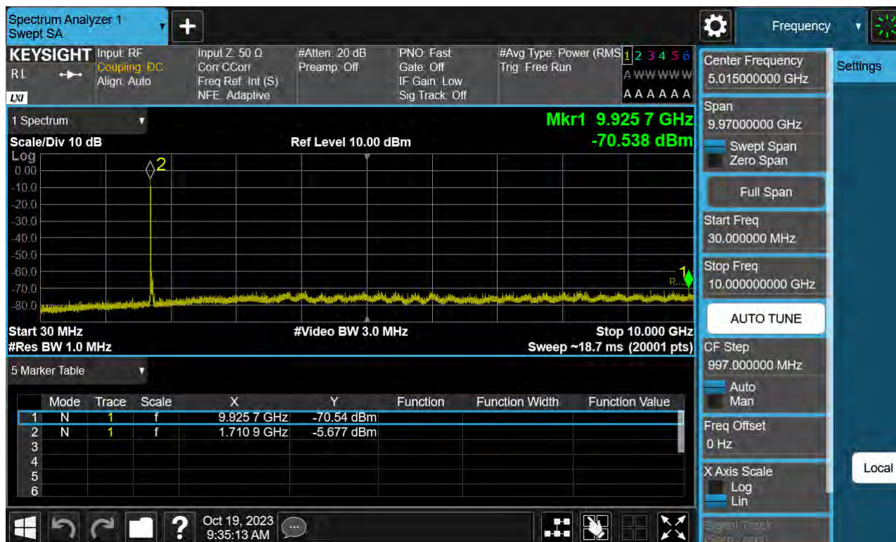
Sub6 n66. Conducted Spurious Plot_1 (345500ch_35 MHz_BPSK_ RB 1_1)
