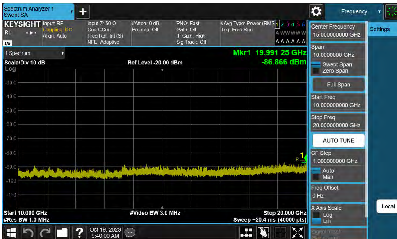
Sub6 n66. Conducted Spurious Plot_2 (349000ch_35 MHz_BPSK_ RB 1_1)
