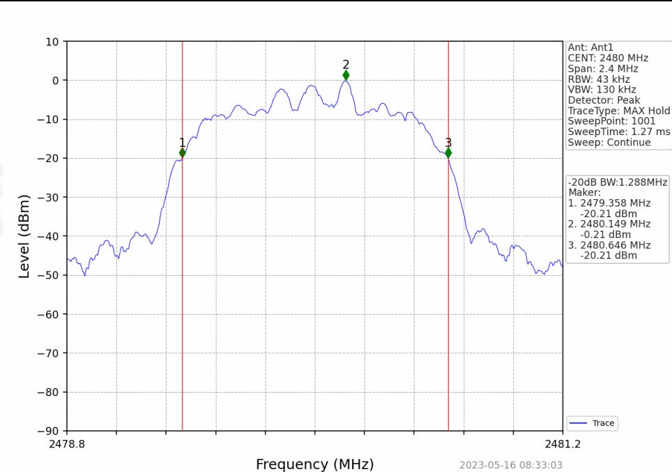
Pi/4DQPSK_2DH5_HCH_2480MHz_Ant1_NTNV
