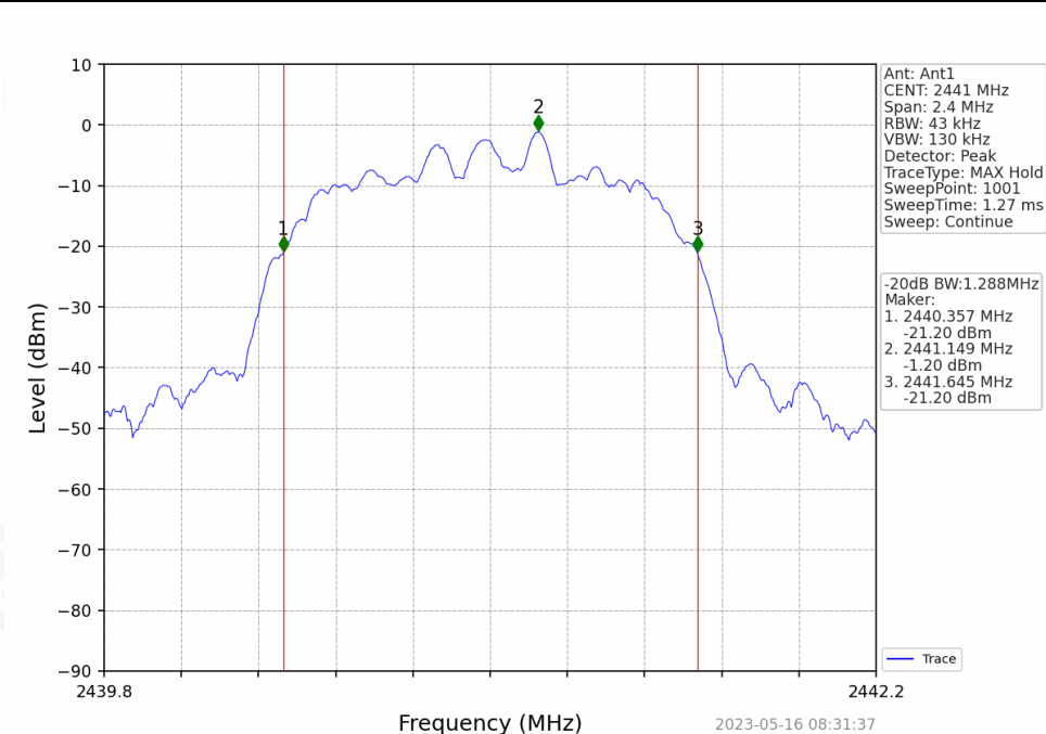
Pi/4DQPSK_2DH5_MCH_2441MHz_Ant1_NTNV
