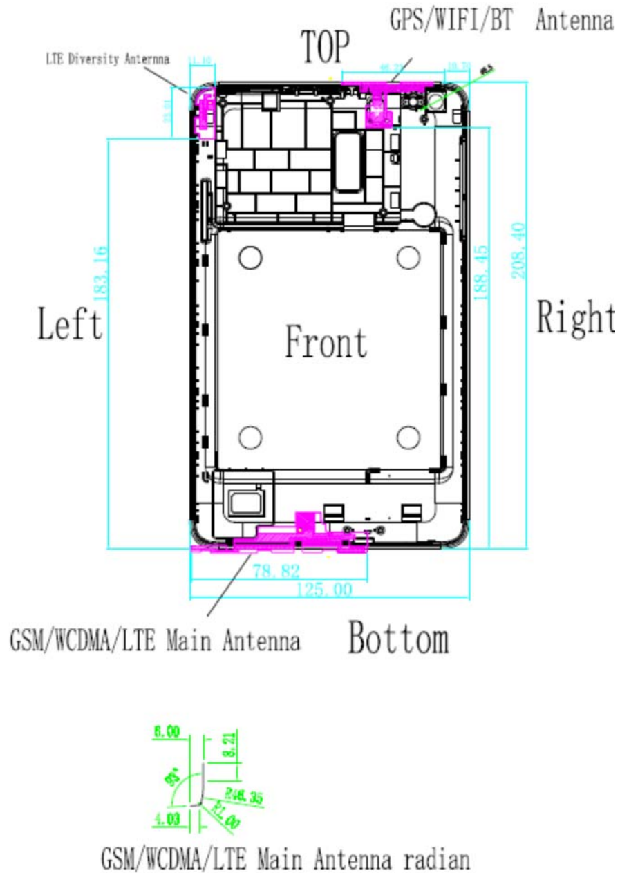
Fig.11.1 EUT Antenna Locations
