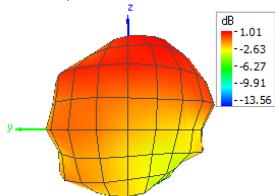
Theta = 90, Phi = 180
