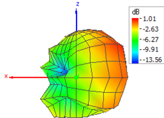
Theta = 90, Phi = 90
