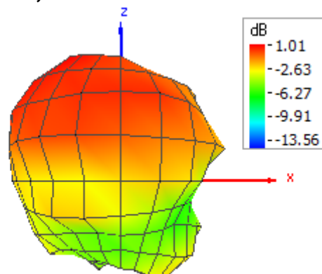
Theta = 90, Phi = 270
