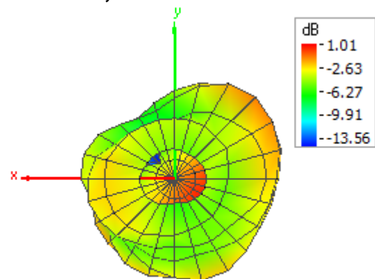
Theta = 180, Phi = 0
