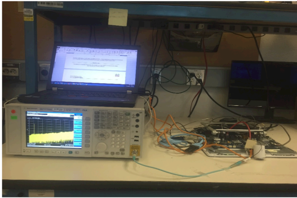
Title: RF Conducted Test Setup
