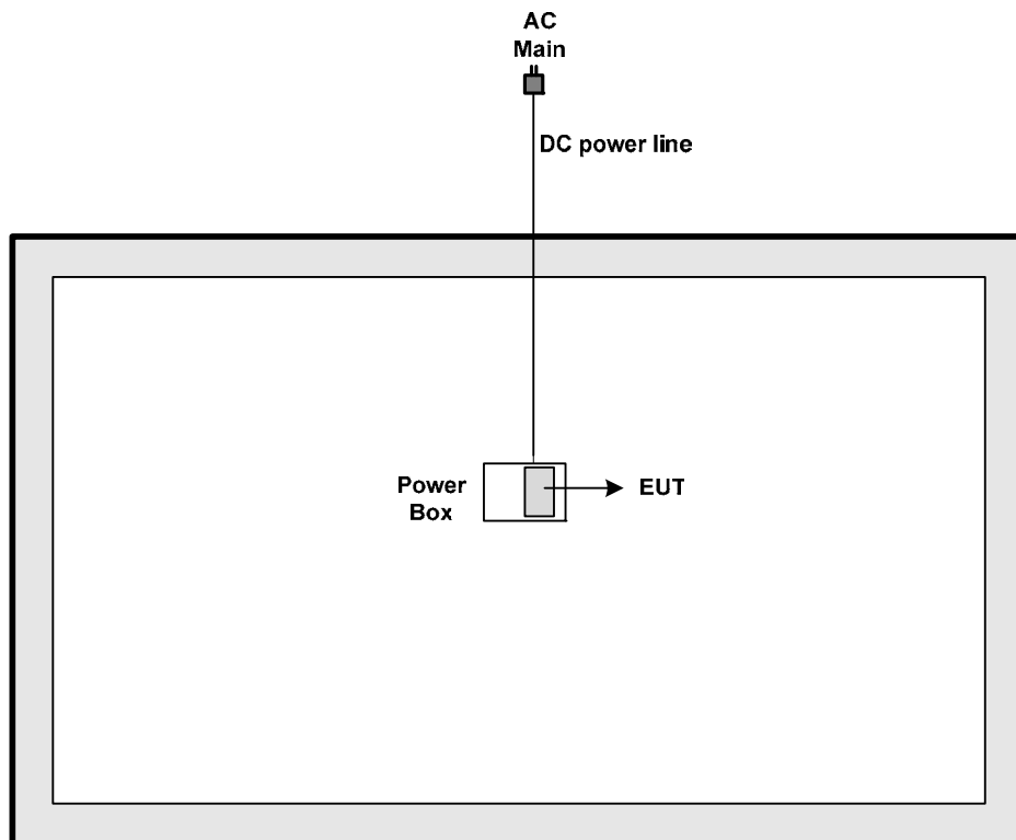
Test Setup Diagram - Radiated Emission (Above 1GHz)
