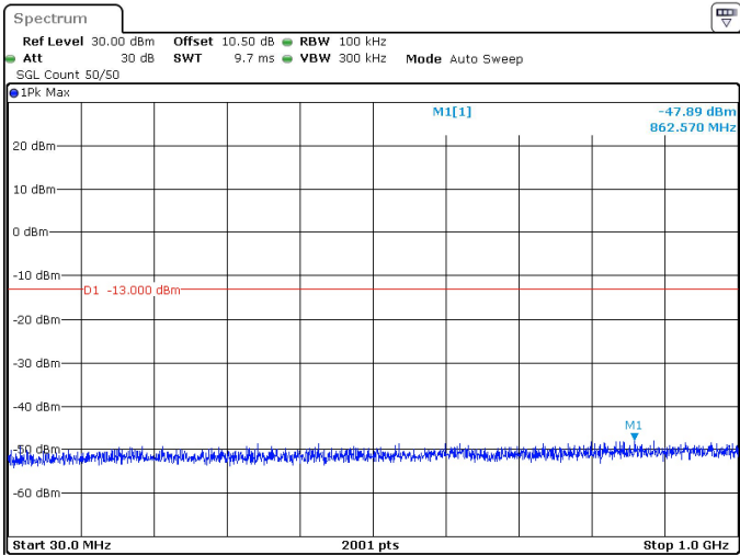
40MHz_30kHz_3500MHz_DFT-s-OFDM QPSK_RB100@0 -47.89 dBm
