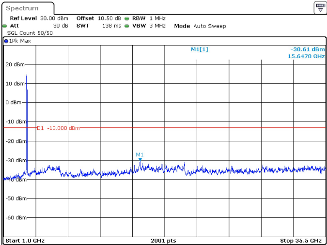
40MHz_30kHz_3500MHz_DFT-s-OFDM QPSK_RB100@0 -30.61 dBm
