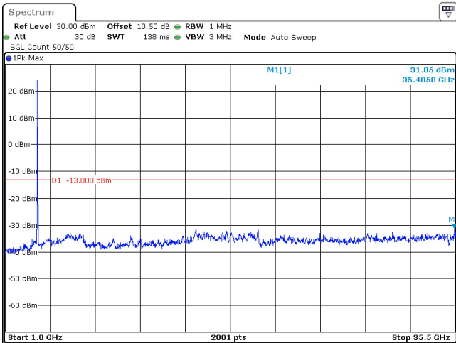
40MHz_30kHz_3500MHz_DFT-s-OFDM QPSK_RB1@0 -31.05 dBm
