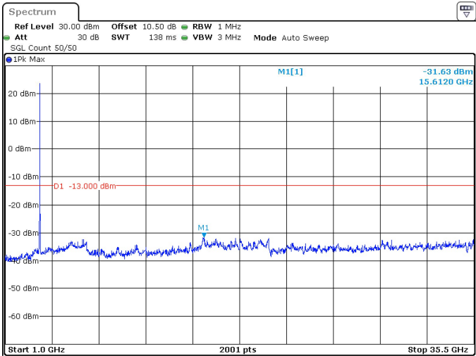
30MHz_30kHz_3535MHz_DFT-s-OFDM QPSK_RB1@77 -31.63 dBm
