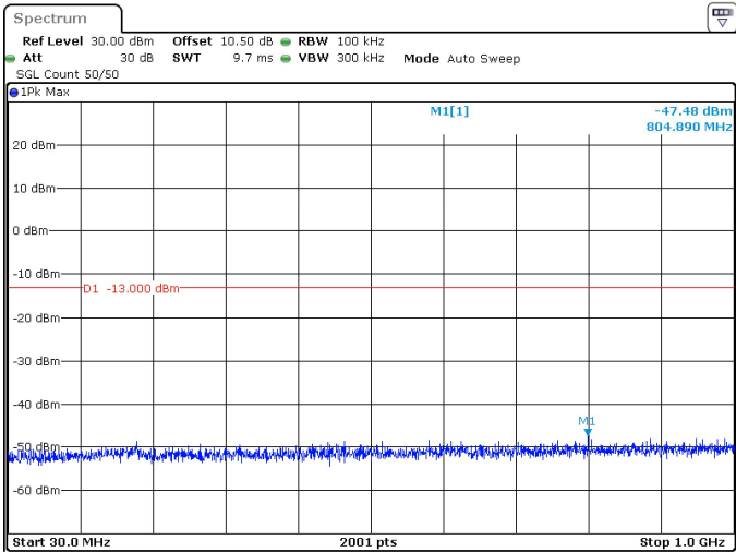
40MHz_30kHz_3500MHz_DFT-s-OFDM QPSK_RB1@105 -47.48 dBm
