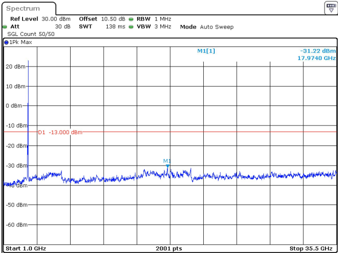
40MHz_30kHz_3500MHz_DFT-s-OFDM QPSK_RB1@105 -31.22 dBm
