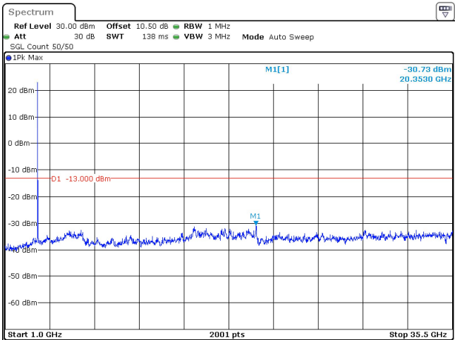
40MHz_30kHz_3530MHz_DFT-s-OFDM QPSK_RB1@0 -30.73 dBm
