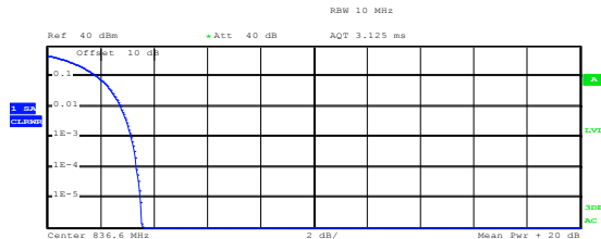
UMTS 850 RMC
