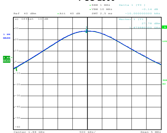
PCS 1900
