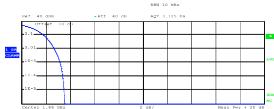
UMTS 1900 RMC
