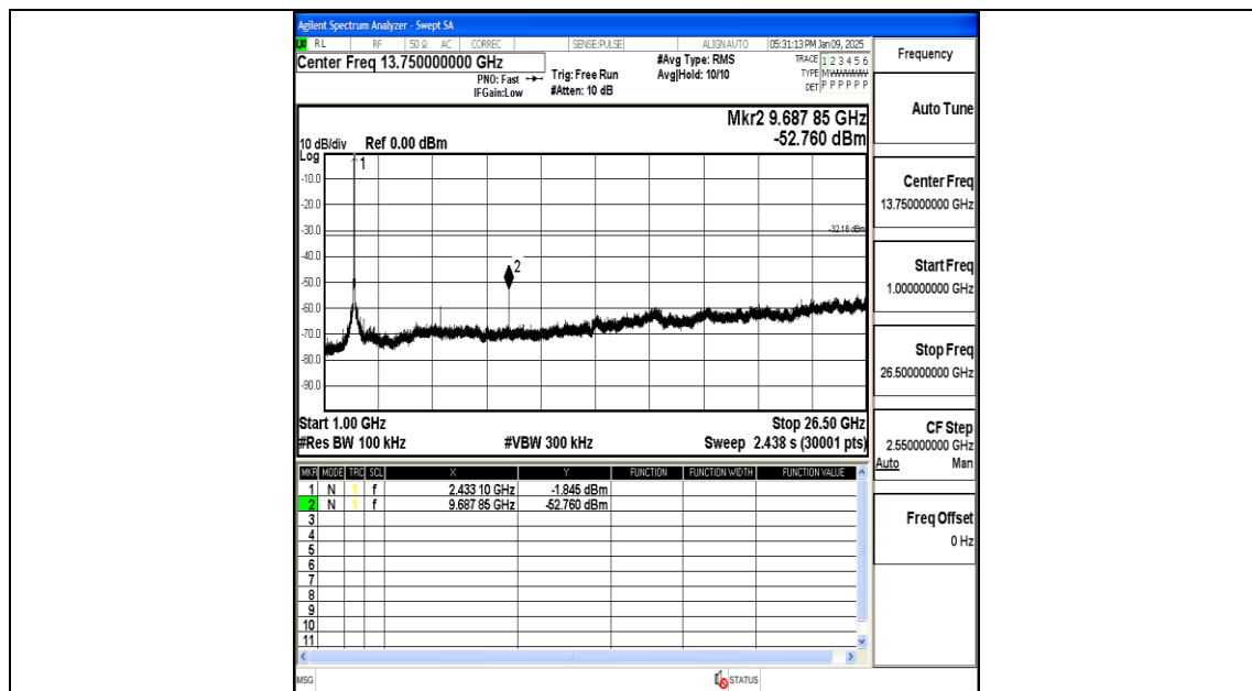
11N40MIMO-Ant2-2422-1000~26500-PASS
