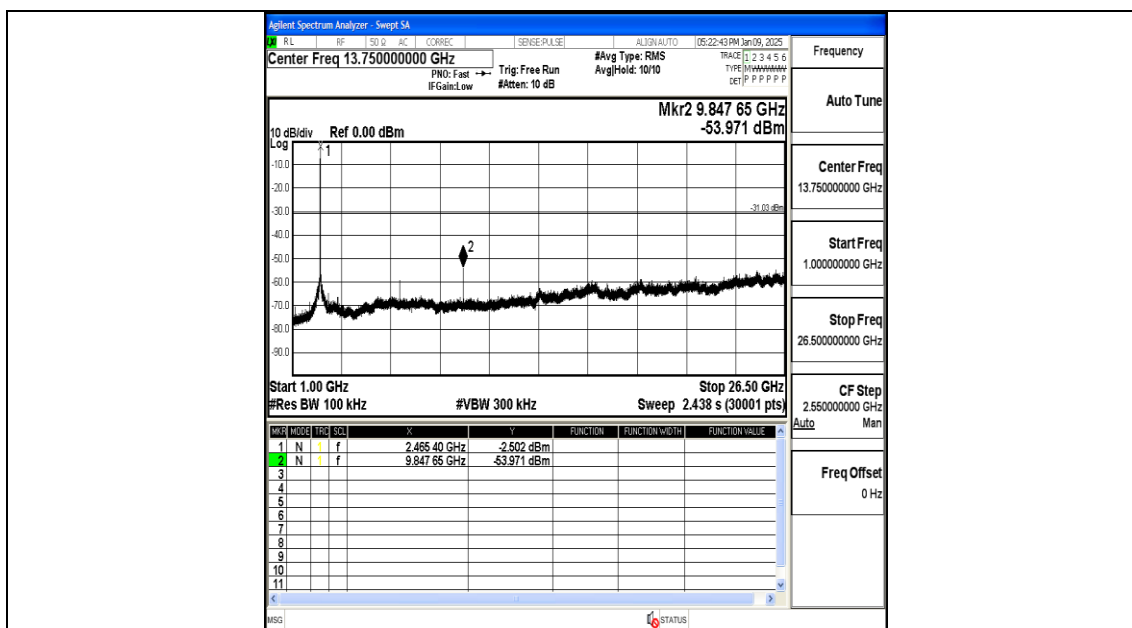
11N20MIMO-Ant2-2462-1000~26500-PASS
