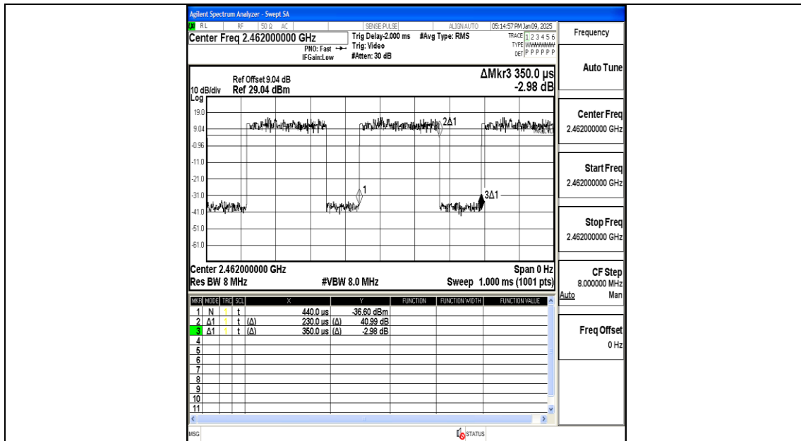
NTNV-11N20MIMO-Ant2-2462
