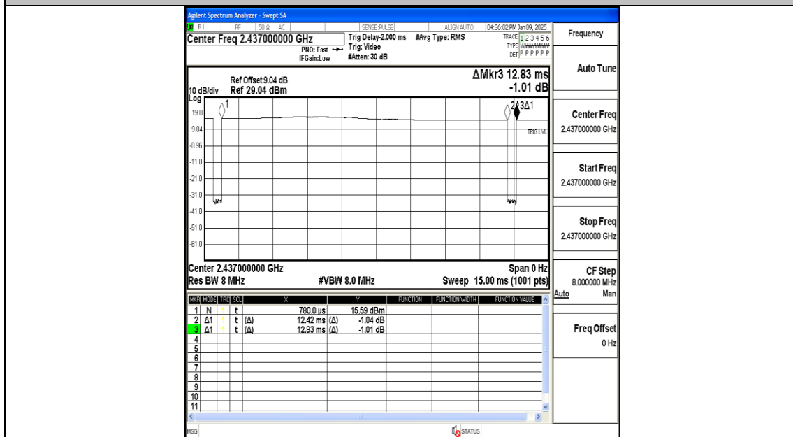
NTNV-11B-Ant2-2437
