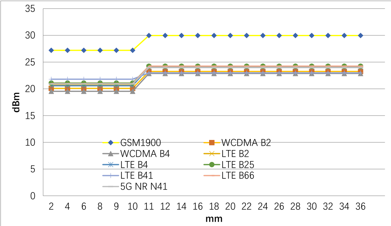
DUT Moving Away the Phantom Output Power:
