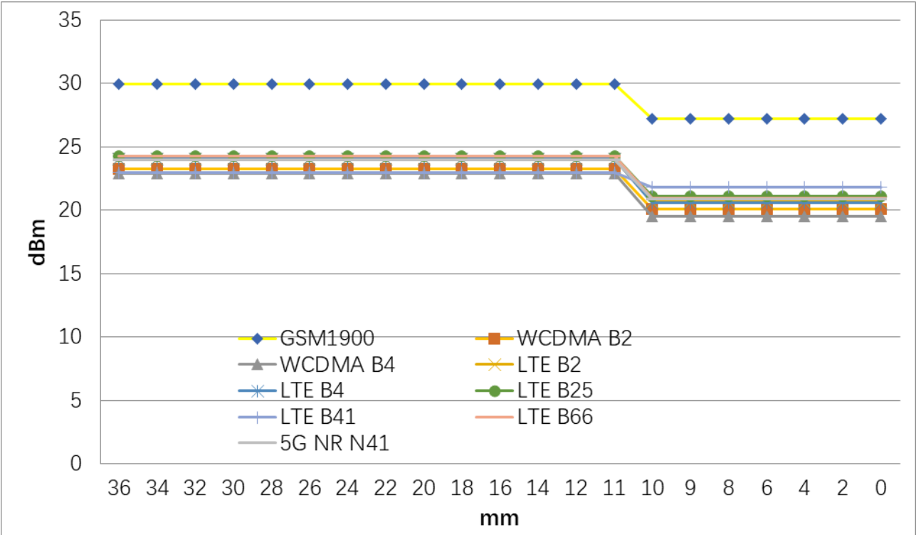
DUT Moving Toward the Phantom Output Power:
