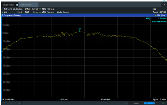
\pi/4 -DQPSK on Channel 00
