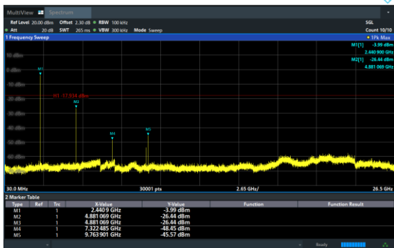
8DPSK on Channel 39
