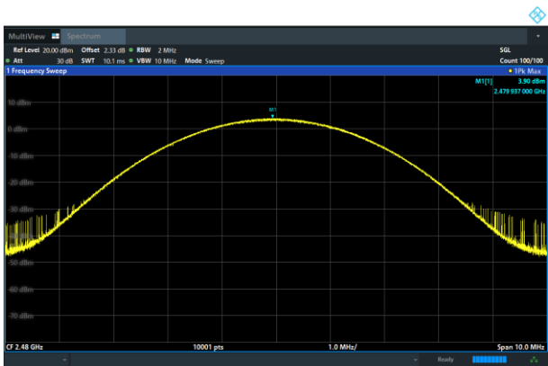
8DPSK on Channel 78
