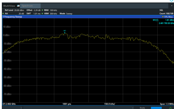
8DPSK on Channel 00
