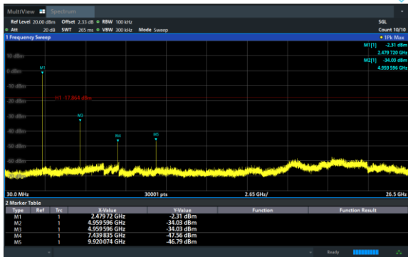
8DPSK on Channel 78
