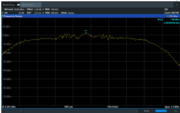
\pi/4 -DQPSK on Channel 39
