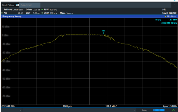
GFSK on Channel 00
