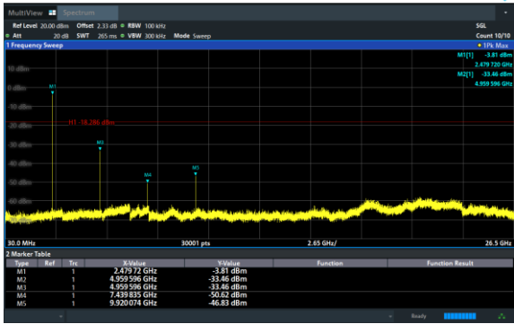
\pi/4 -DQPSK on Channel 78
