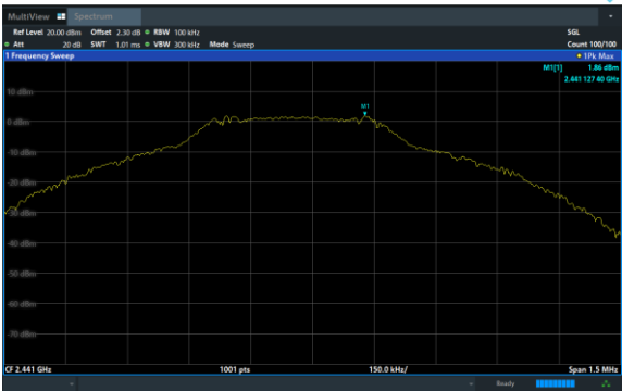
GFSK on Channel 39
