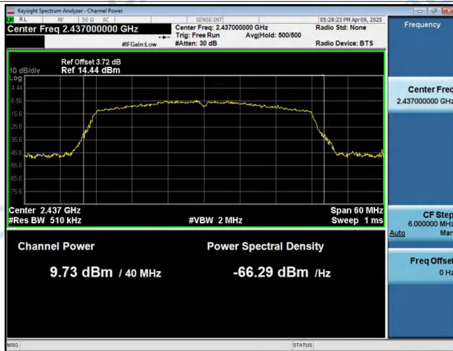
MAX__Output_Power_NVNT_ANT1_802_11n(HT40)_2437
