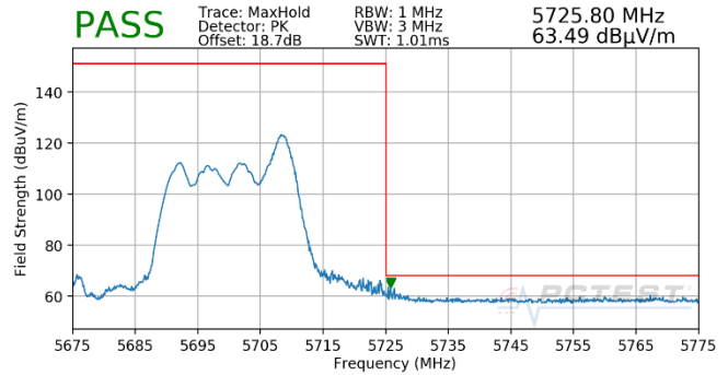
Plot 7-524. SDM (Pk, RU26, Index 8, Ch.140, MCS11)
