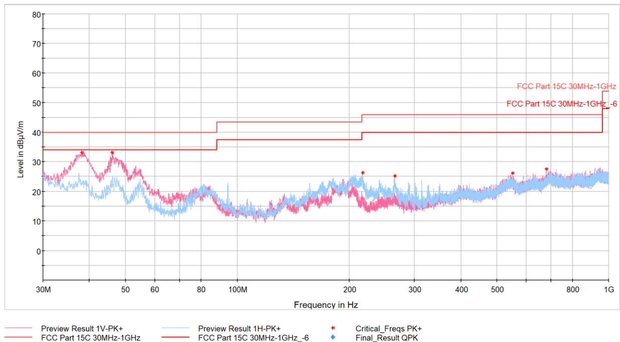
Plot 7-567. RSE below 1GHz CDD (RU26 – Ch.56), with AC/DC Adapter
