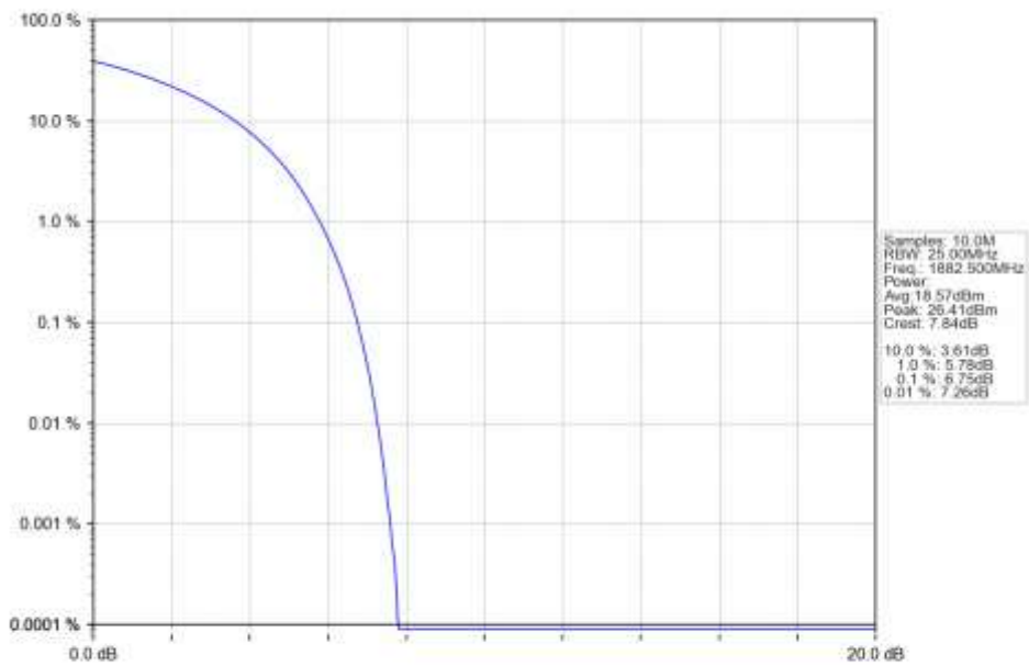
n25_30kHz_SISO_NTNV_20MHz_CP-OFDM_QPSK_1882.5MHz_Outer_Full_Ant1
