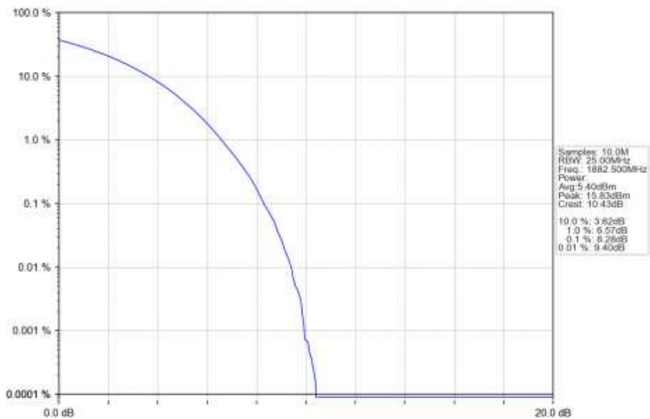
n25_15kHz_SISO_NTNV_20MHz_CP-OFDM_256_QAM_1882.5MHz_Outer_Full_Ant1
