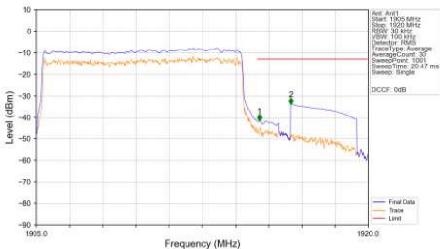
n25_15kHz_SISO_NTNV_10MHz_DFT-s-OFDM_QPSK_1910MHz_Outer_Full_Ant1
