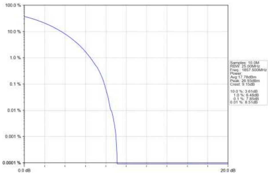
n25_30kHz_SISO_NTNV_15MHz_CP-OFDM_64_QAM_1857.5MHz_Outer_Full_Ant1
