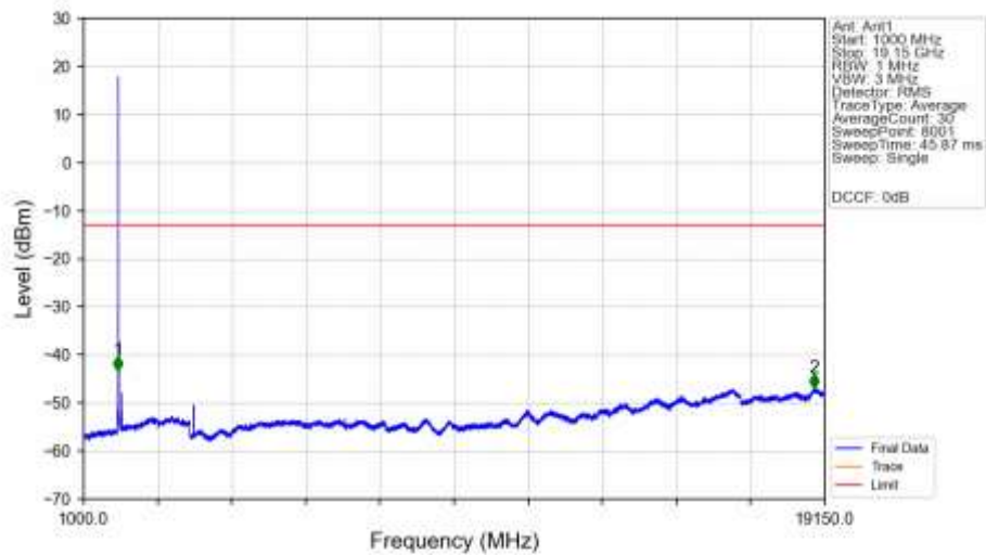
n25_30kHz_SISO_NTNV_10MHz_DFT-s-OFDM_QPSK_1855MHz_Edge_1RB_Left_Ant1
