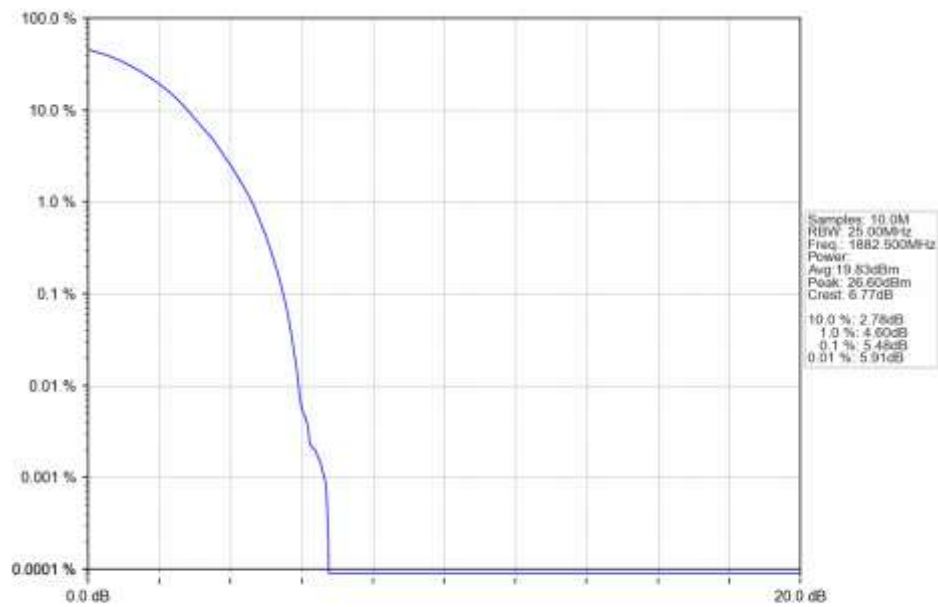
n25_30kHz_SISO_NTNV_15MHz_DFT-s-OFDM_64_QAM_1882.5MHz_Outer_Full_Ant1
