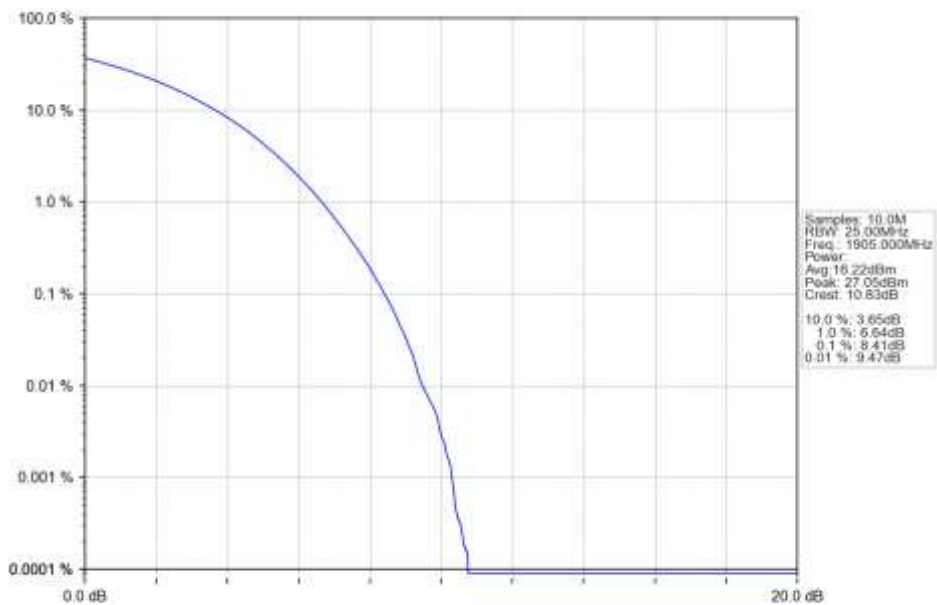
n25_15kHz_SISO_NTNV_20MHz_CP-OFDM_256_QAM_1905MHz_Outer_Full_Ant1
