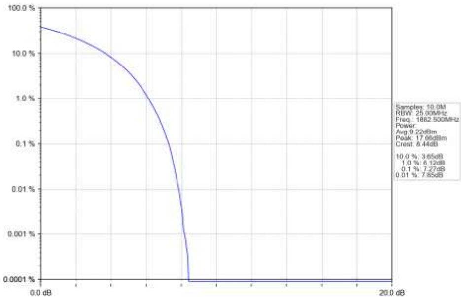
n25_15kHz_SISO_NTNV_20MHz_CP-OFDM_QPSK_1882.5MHz_Outer_Full_Ant1
