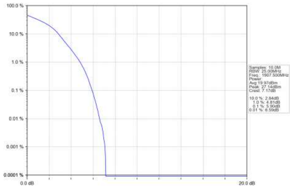
n25_30kHz_SISO_NTNV_15MHz_DFT-s-OFDM_16_QAM_1907.5MHz_Outer_Full_Ant1
