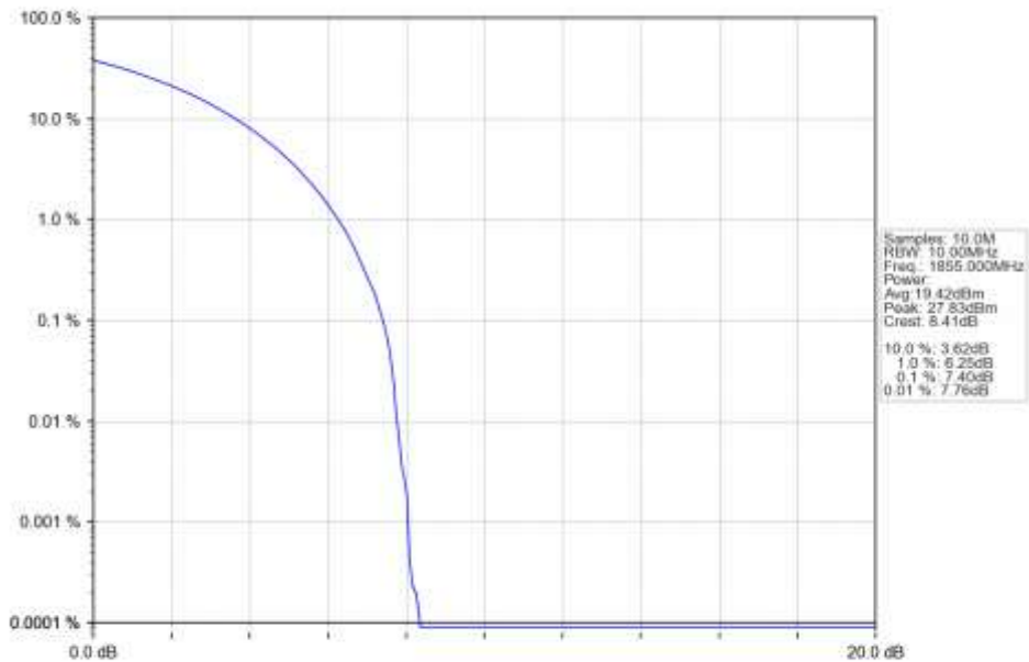
n25_30kHz_SISO_NTNV_10MHz_CP-OFDM_QPSK_1855MHz_Outer_Full_Ant1
