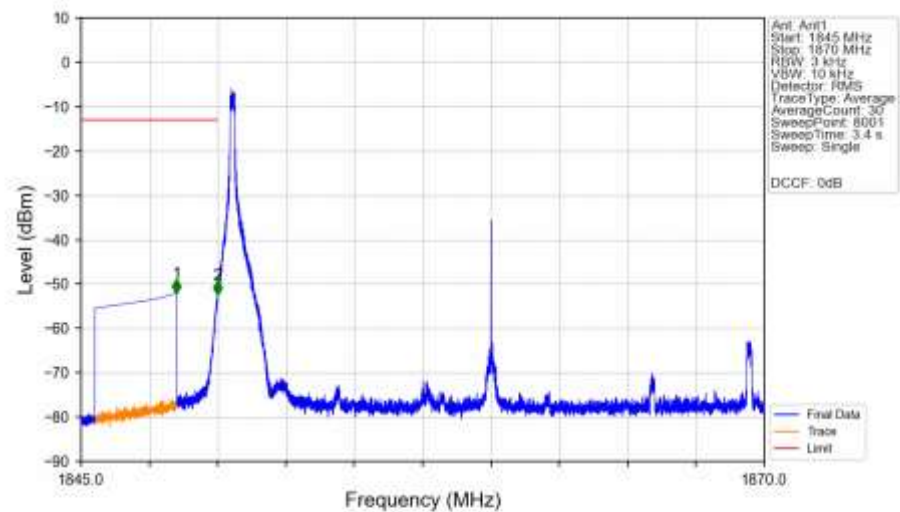
n25_15kHz_SISO_NTNV_20MHz_DFT-s-OFDM_QPSK_1860MHz_Edge_1RB_Left_Ant1
