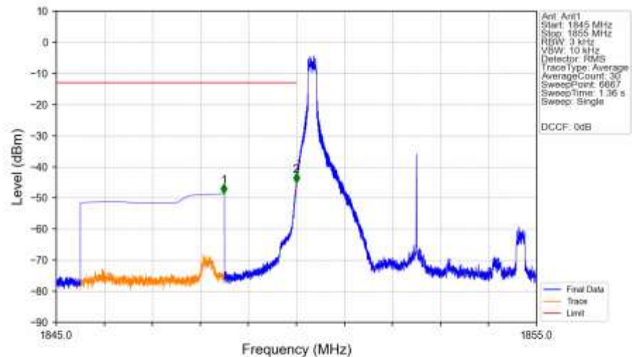
n25_15kHz_SISO_NTNV_5MHz_DFT-s-OFDM_QPSK_1852.5MHz_Edge_1RB_Left_Ant1
