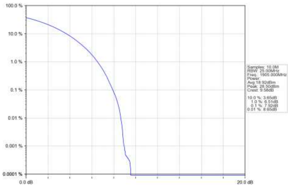
n25_15kHz_SISO_NTNV_20MHz_CP-OFDM_64_QAM_1905MHz_Outer_Full_Ant1
