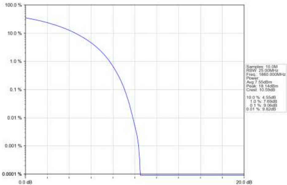
n25_15kHz_SISO_NTNV_20MHz_CP-OFDM_QPSK_1860MHz_Outer_Full_Ant1
