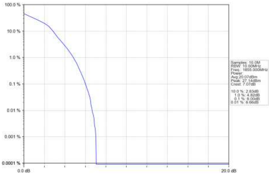
n25_30kHz_SISO_NTNV_10MHz_DFT-s-OFDM_16_QAM_1855MHz_Outer_Full_Ant1
