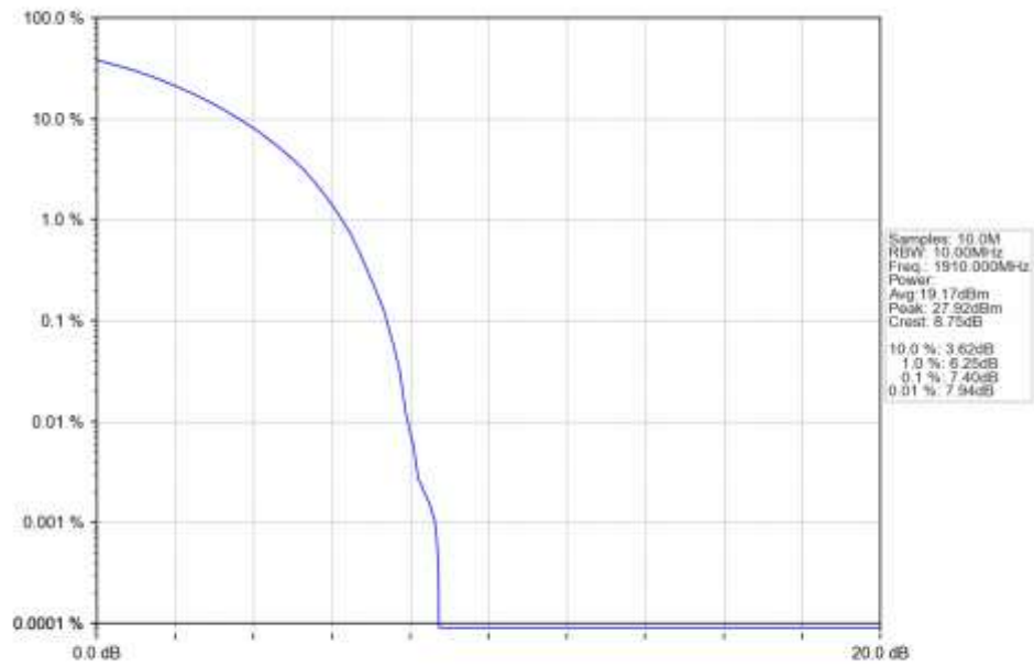
n25_30kHz_SISO_NTNV_10MHz_CP-OFDM_64_QAM_1910MHz_Outer_Full_Ant1
