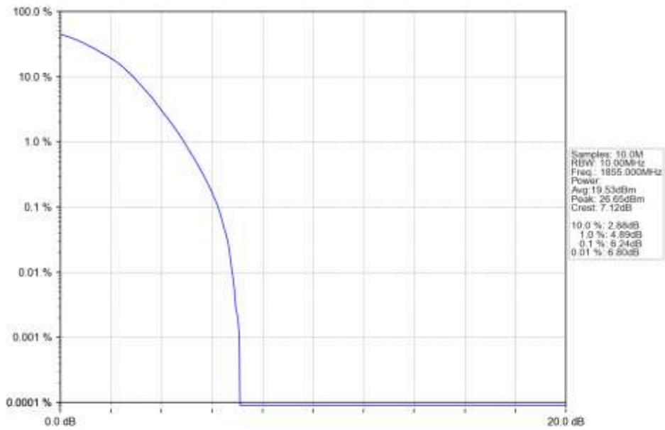
n25_30kHz_SISO_NTNV_10MHz_DFT-s-OFDM_64_QAM_1855MHz_Outer_Full_Ant1
