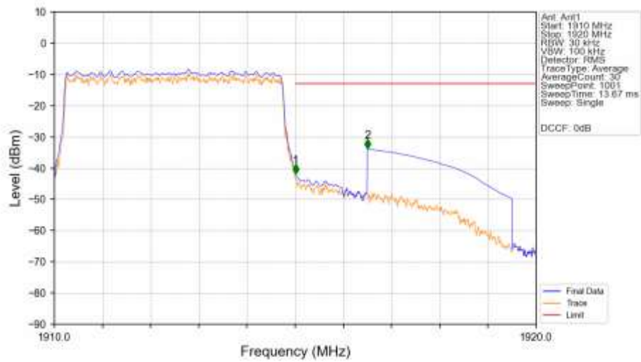
n25_15kHz_SISO_NTNV_5MHz_DFT-s-OFDM_QPSK_1912.5MHz_Outer_Full_Ant1
