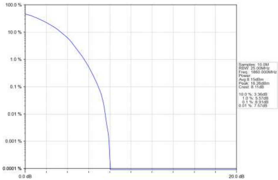
n25_15kHz_SISO_NTNV_20MHz_DFT-s-OFDM_64_QAM_1860MHz_Outer_Full_Ant1
