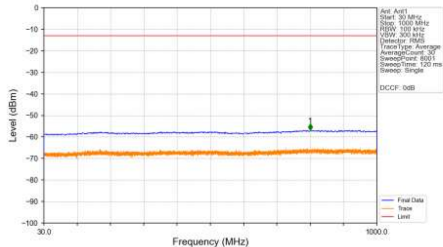
n25_15kHz_SISO_NTNV_5MHz_DFT-s-OFDM_QPSK_1852.5MHz_Edge_1RB_Left_Ant1
