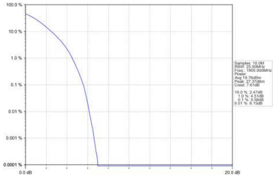
n25_30kHz_SISO_NTNV_20MHz_DFT-s-OFDM_QPSK_1905MHz_Outer_Full_Ant1
