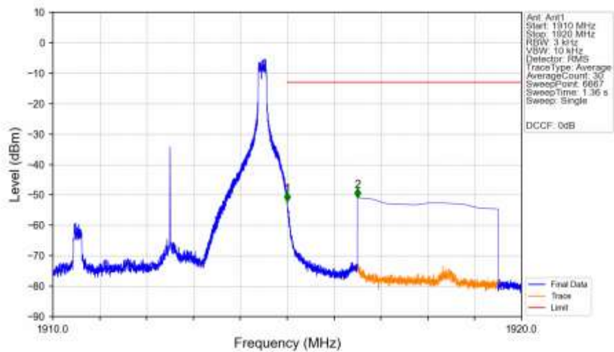
n25_15kHz_SISO_NTNV_5MHz_DFT-s-OFDM_QPSK_1912.5MHz_Inner_1RB_Right_Ant1
