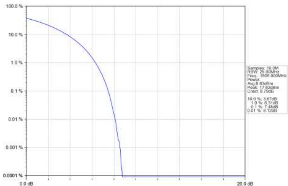
n25_15kHz_SISO_NTNV_20MHz_CP-OFDM_QPSK_1905MHz_Outer_Full_Ant1
