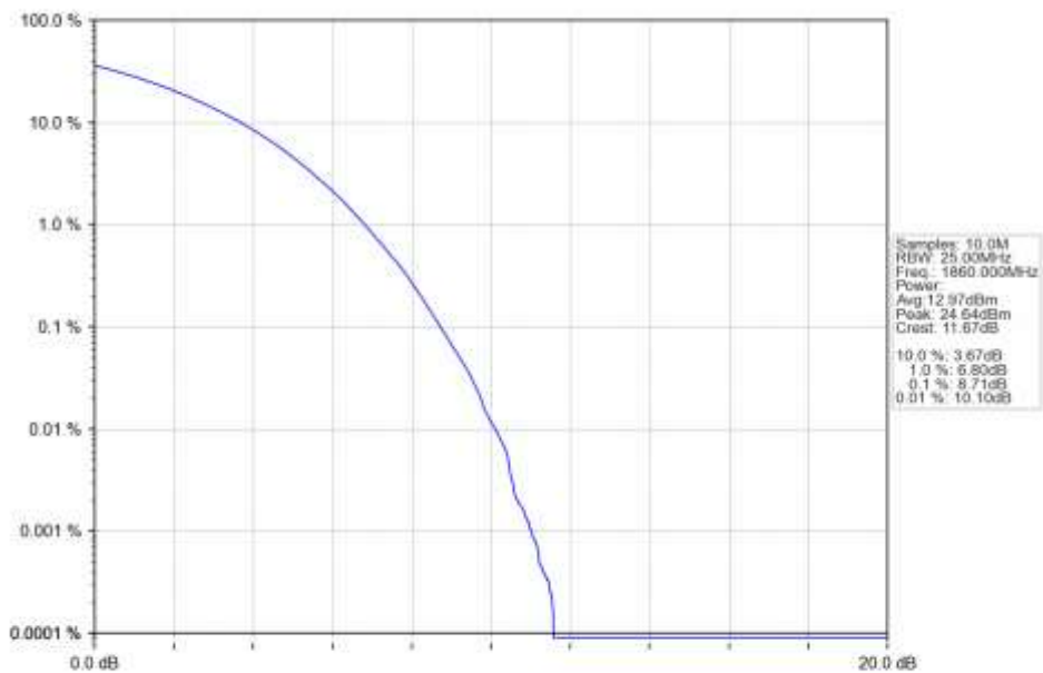
n25_15kHz_SISO_NTNV_20MHz_CP-OFDM_256_QAM_1860MHz_Outer_Full_Ant1
