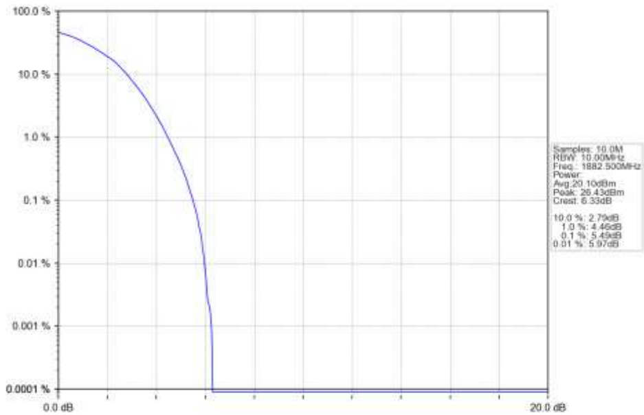
n25_30kHz_SISO_NTNV_10MHz_DFT-s-OFDM_64_QAM_1882.5MHz_Outer_Full_Ant1
