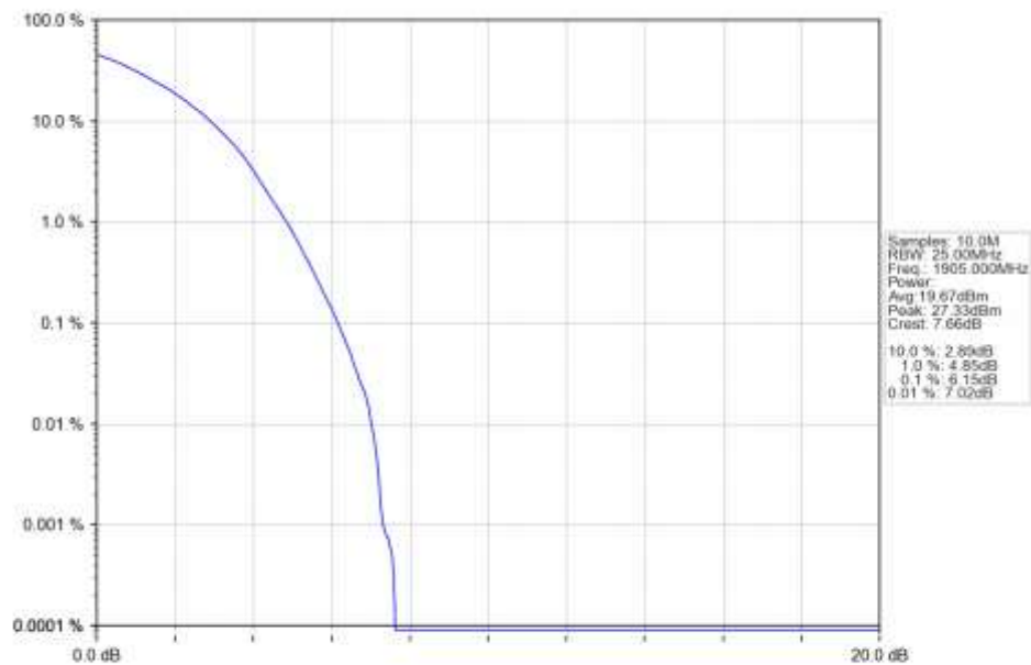
n25_30kHz_SISO_NTNV_20MHz_DFT-s-OFDM_16_QAM_1905MHz_Outer_Full_Ant1
