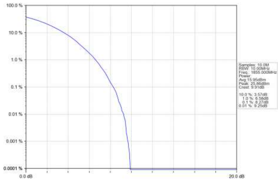
n25_30kHz_SISO_NTNV_10MHz_CP-OFDM_256_QAM_1855MHz_Outer_Full_Ant1
