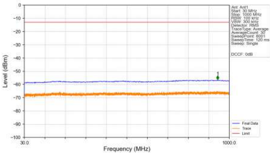
n25_30kHz_SISO_NTNV_10MHz_DFT-s-OFDM_QPSK_1855MHz_Edge_1RB_Left_Ant1
