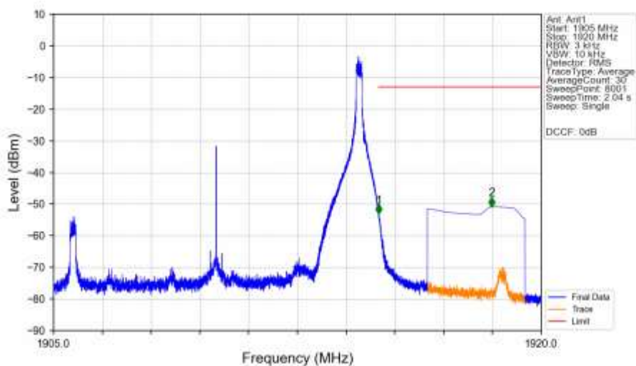
n25_15kHz_SISO_NTNV_10MHz_DFT-s-OFDM_QPSK_1910MHz_Inner_1RB_Right_Ant1
