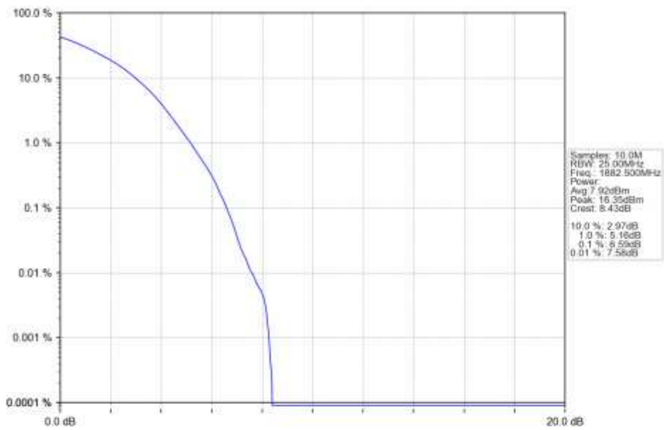
n25_15kHz_SISO_NTNV_20MHz_DFT-s-OFDM_256_QAM_1882.5MHz_Outer_Full_Ant1
