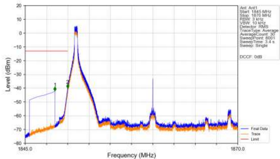
n25_30kHz_SISO_NTNV_20MHz_DFT-s-OFDM_QPSK_1860MHz_Edge_1RB_Left_Ant1
