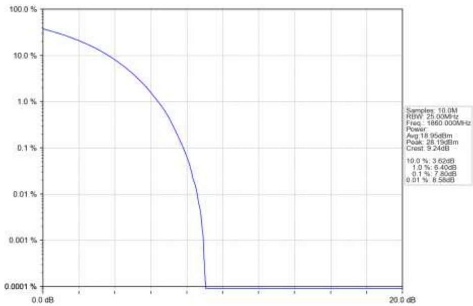
n25_30kHz_SISO_NTNV_20MHz_CP-OFDM_QPSK_1860MHz_Outer_Full_Ant1
