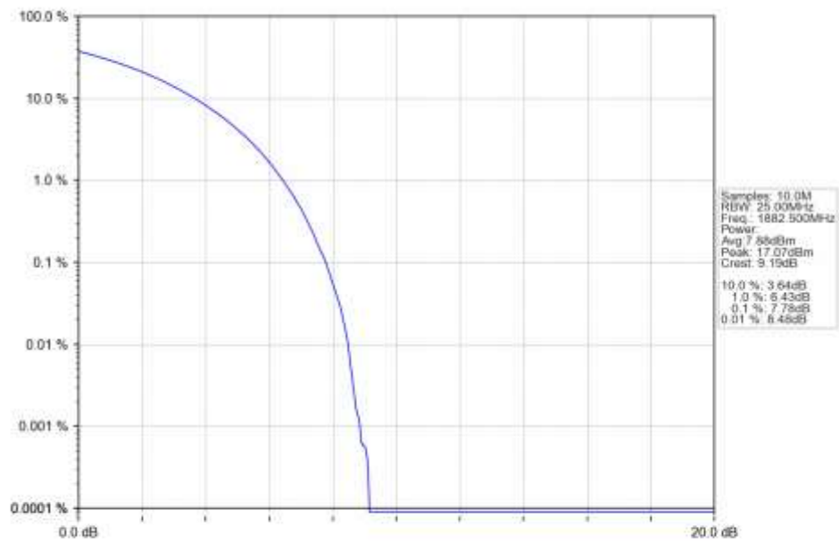
n25_15kHz_SISO_NTNV_20MHz_CP-OFDM_64_QAM_1882.5MHz_Outer_Full_Ant1
