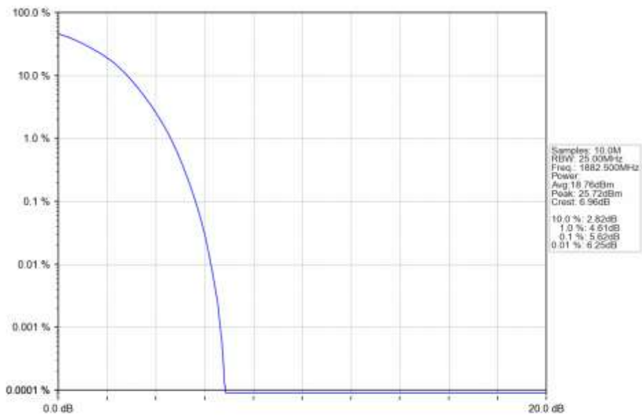
n25_30kHz_SISO_NTNV_20MHz_DFT-s-OFDM_64_QAM_1882.5MHz_Outer_Full_Ant1
