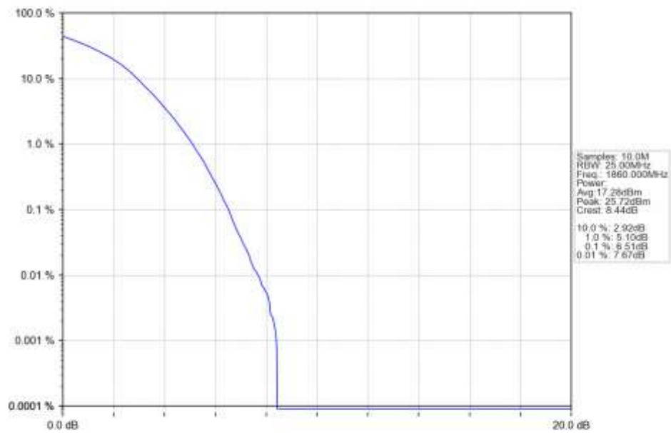
n25_30kHz_SISO_NTNV_20MHz_DFT-s-OFDM_256_QAM_1860MHz_Outer_Full_Ant1
