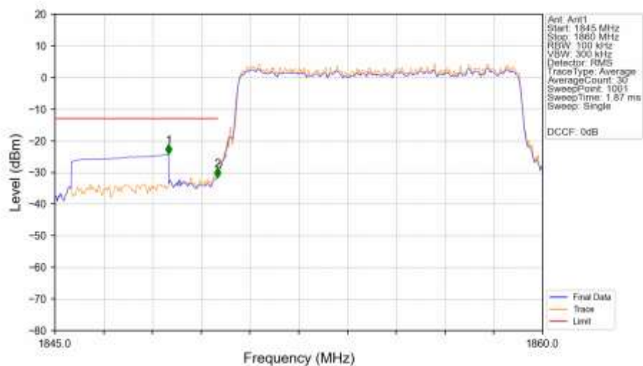
n25_30kHz_SISO_NTNV_10MHz_DFT-s-OFDM_QPSK_1855MHz_Outer_Full_Ant1
