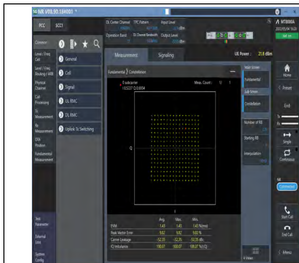
1-N77-3700-3980-PC2-30-100-M-5-DFT-256QAM-O uter_Full-270@0-Ant1-see graph-PASS
