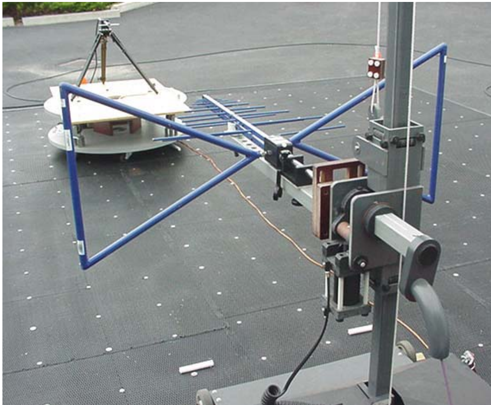
Substitution Dipole antenna
