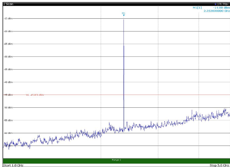
Channel: TOP, Modulation: QPSK, BW=5MHz, Range: 1GHz - 5GHz, Polarization: Vertical
