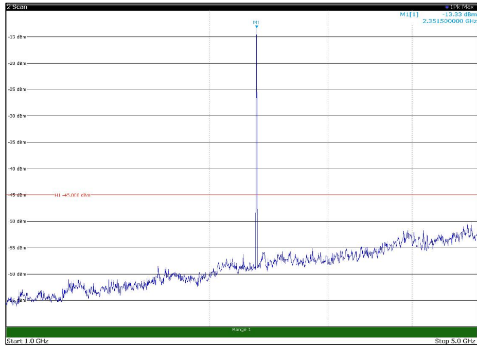
Channel: TOP, Modulation: 64QAM, BW=5MHz, Range: 1GHz - 5GHz, Polarization: Horizontal
