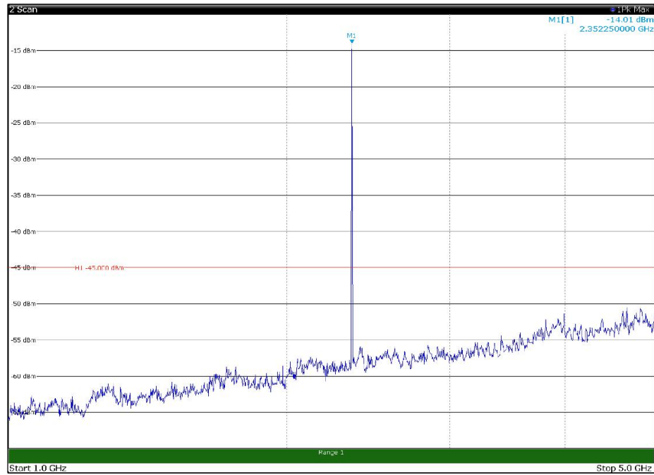
Channel: TOP, Modulation: QPSK, BW=5MHz, Range: 1GHz - 5GHz, Polarization: Horizontal
