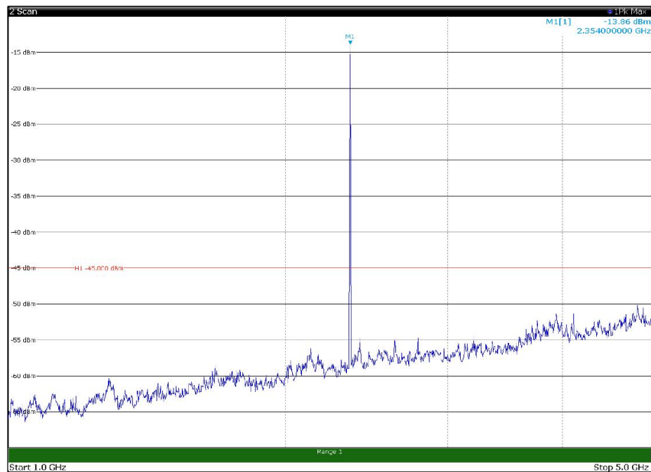
Channel: TOP, Modulation: 64QAM, BW=5MHz, Range: 1GHz - 5GHz, Polarization: Vertical
