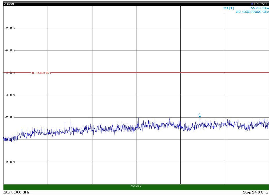
Channel: BOTTOM, Modulation: 16QAM, BW=5MHz, Range: 18GHz - 24GHz, Polarization: Horizontal
