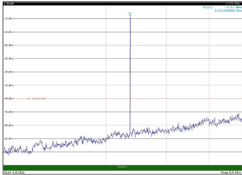
Channel: MIDDLE, Modulation: QPSK, BW=5MHz, Range: 1GHz - 5GHz, Polarization: Horizontal
