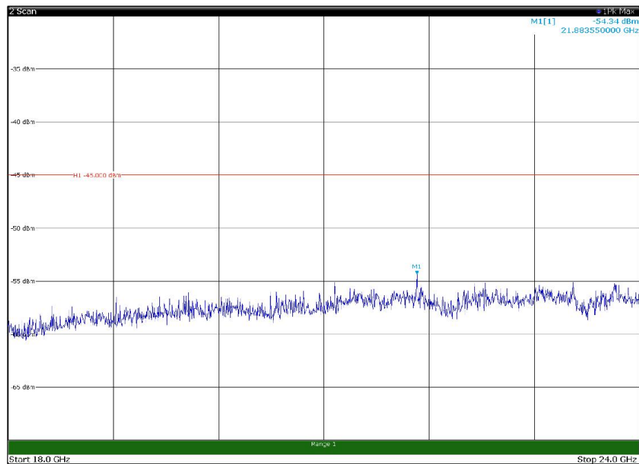
Channel: BOTTOM, Modulation: 16QAM, BW=5MHz, Range: 18GHz - 24GHz, Polarization: Vertical
