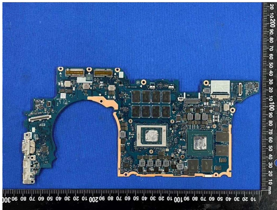
MAIN BOARD TOP VIEW (WITHOUT SHIELDING)(with GPU version)
