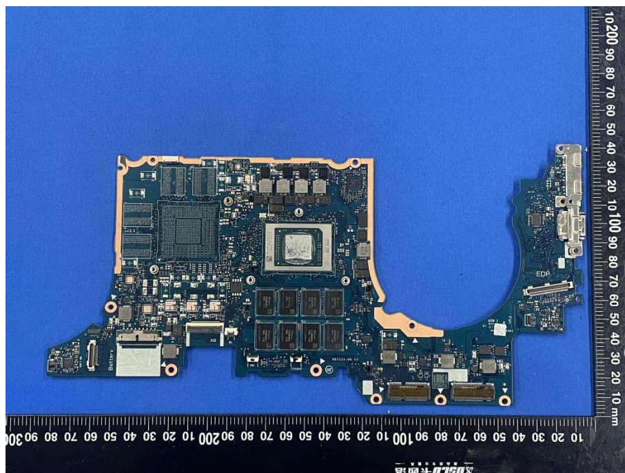
MAIN BOARD TOP VIEW (WITHOUT SHIELDING)(without GPU version)
