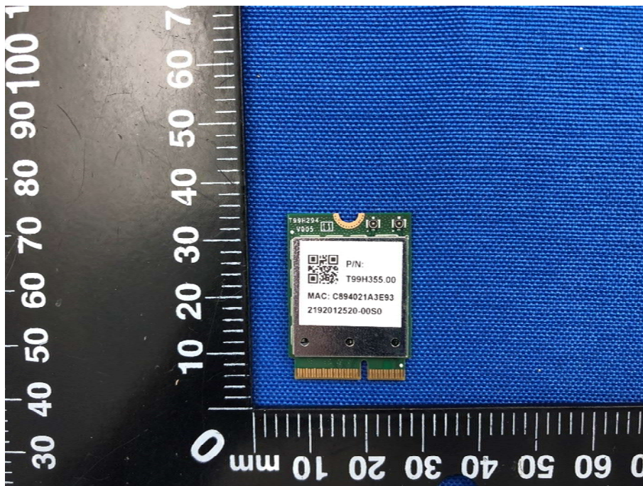
RF MODULE TOP VIEW(WITH SHIELDING)
