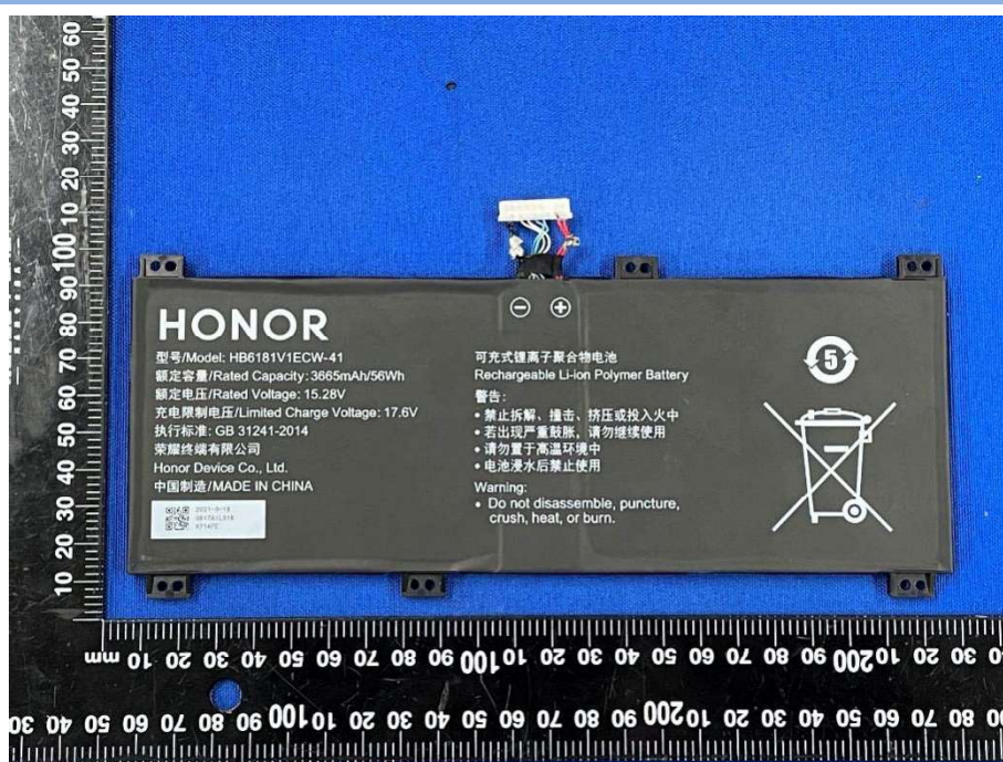
Battery Photo 2 (FRONT)
