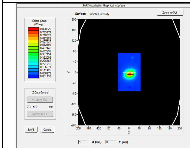
SURFACE SAR
