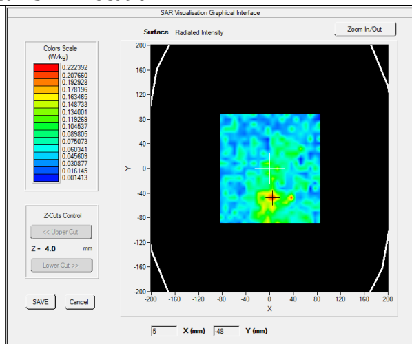
SURFACE SAR
