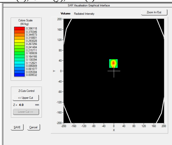
VOLUME SAR
