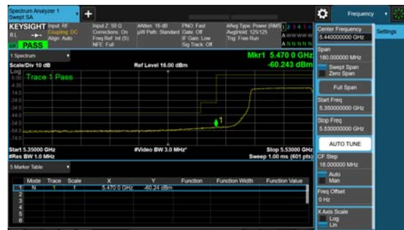
Antenna B
