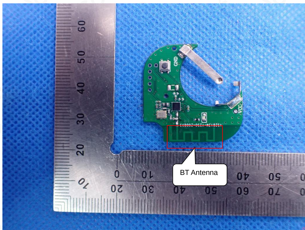
INTERNAL VIEW-4 OF EUT(K11)
