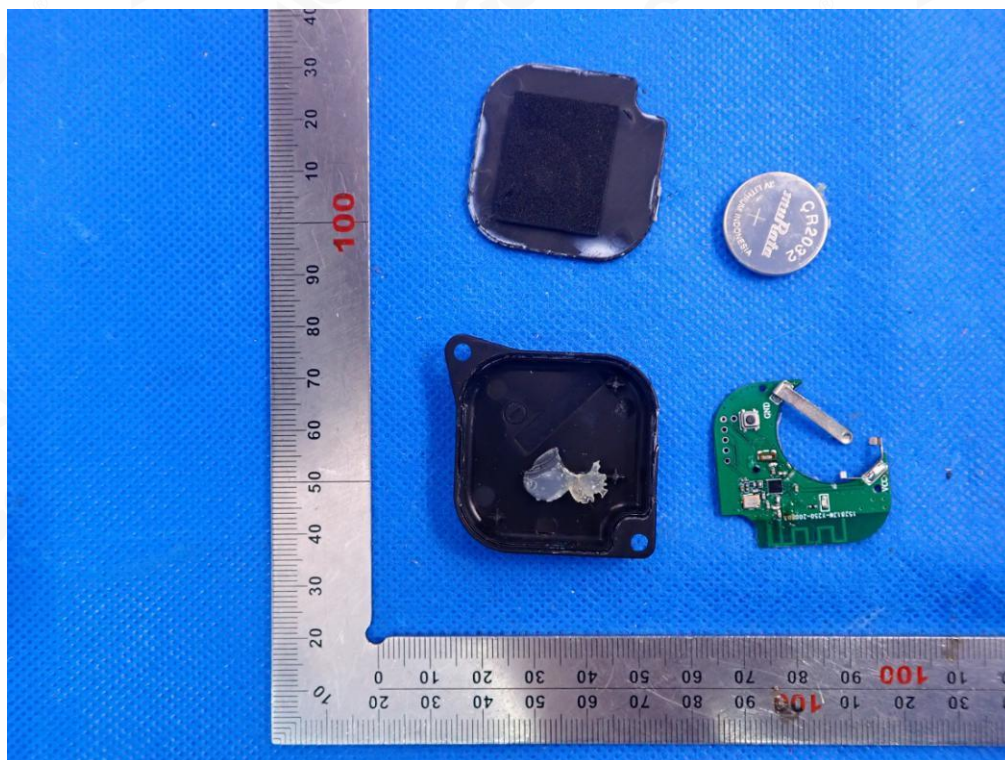
INTERNAL VIEW-1 OF EUT(K12)
