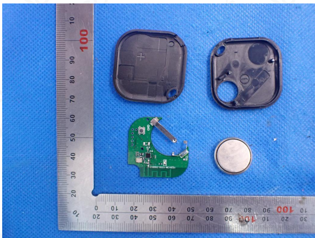
INTERNAL VIEW-2 OF EUT(K11)
