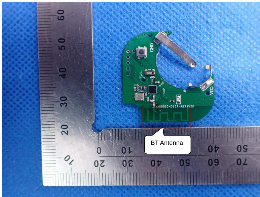
INTERNAL VIEW-3 OF EUT(K12)
