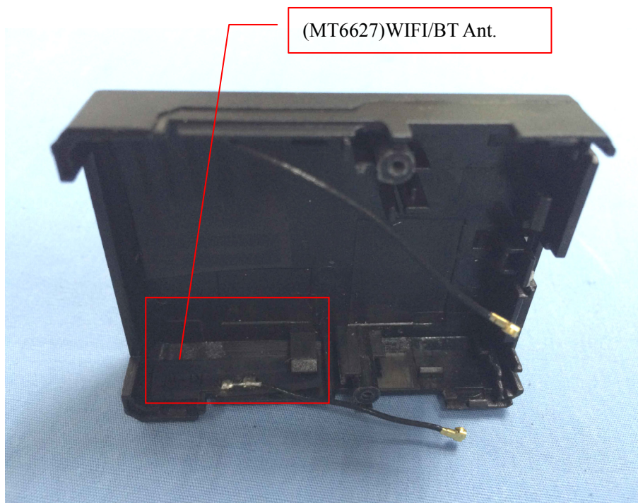
Solder Board-Component View 16
