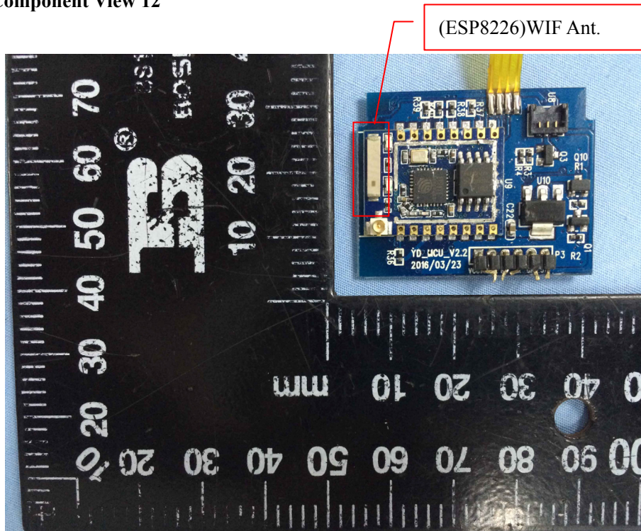
Solder Board-Component View 12
