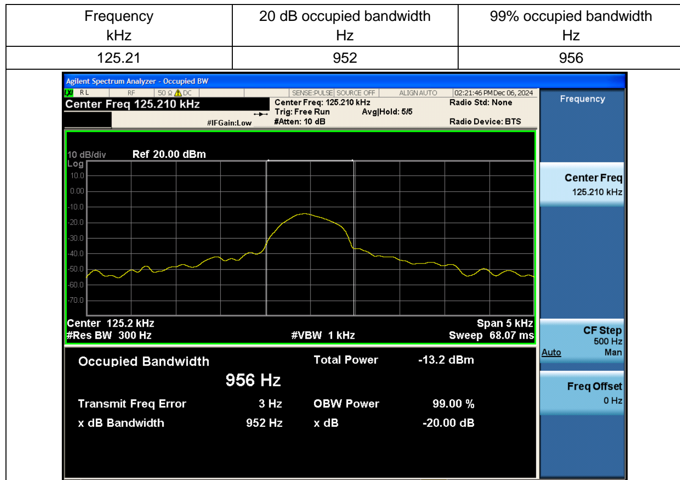
Coil 1
