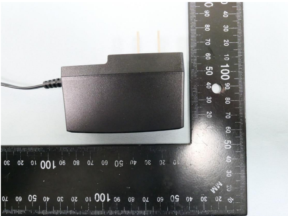
(8) EUT Photo (Brand: tp-link, M/N: T120200-2B1)
