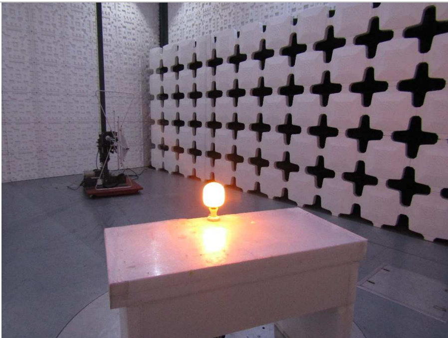
Radiated electromagnetic disturbance (30 MHz -1000MHz)
