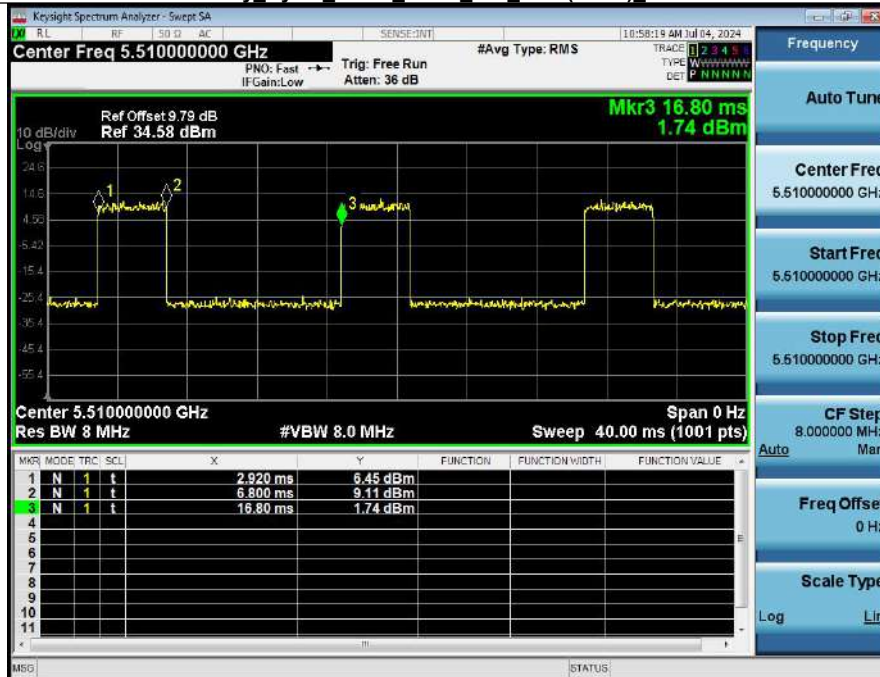
Duty Cycle_NVNT_ANT1_802_11ax(HE40)_5510
