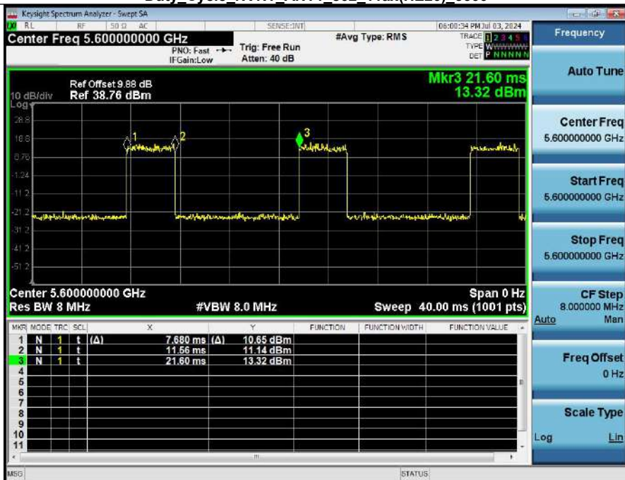
Duty Cycle_NVNT_ANT1_802_11ax(HE20)_5600
