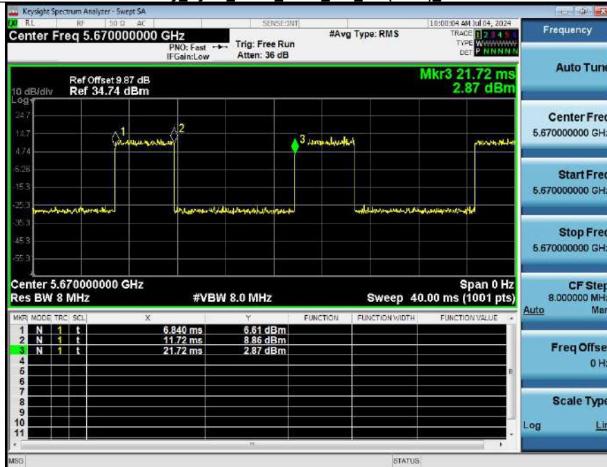
Duty_Cycle_NVNT_ANT1_802_11n(HT40)_5670
