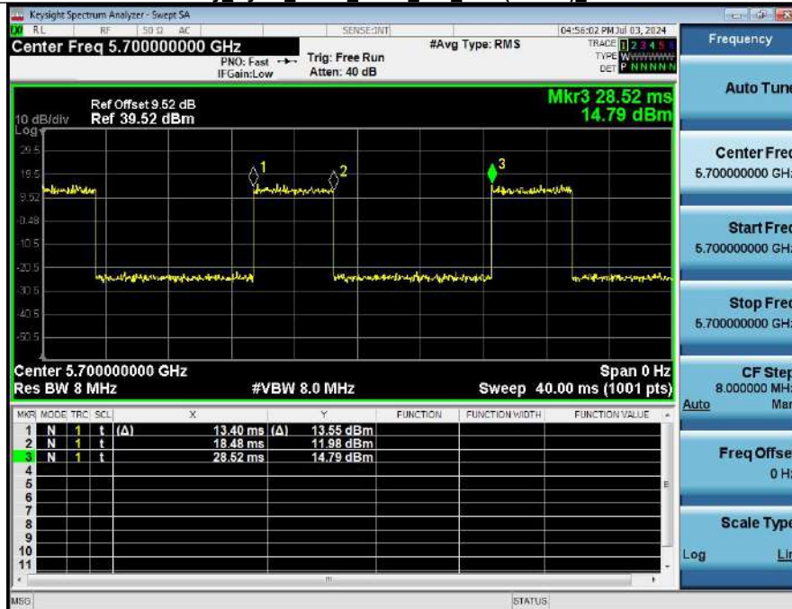
Duty_Cycle_NVNT_ANT1_802_11ac(VHT20)_5700
