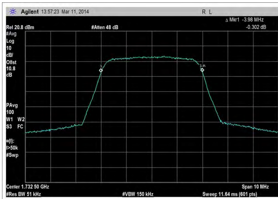
UL_1710-1755MHz_41AWGN_output
