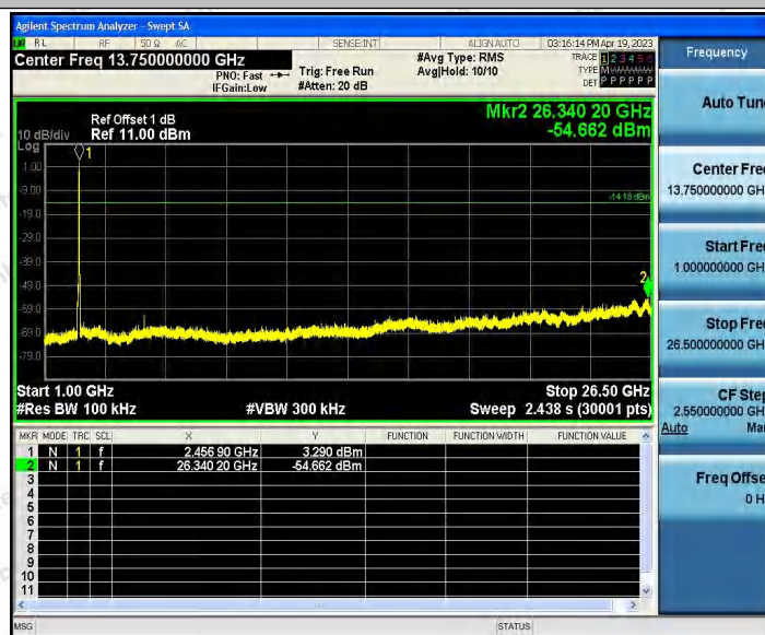
11N20_Ant2_2462_0~Reference
