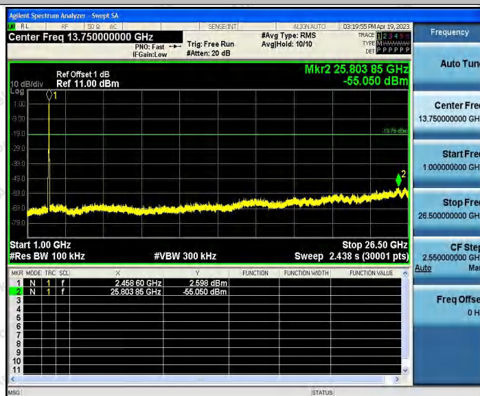
11N40_Ant2_2452_0~Reference
