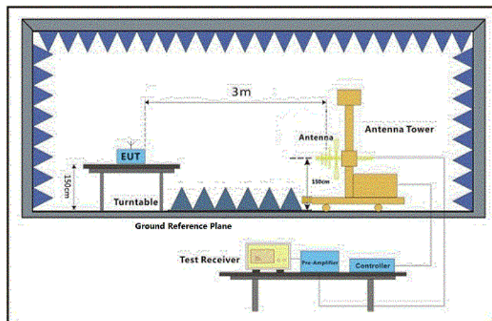
30MHz-1GHz
