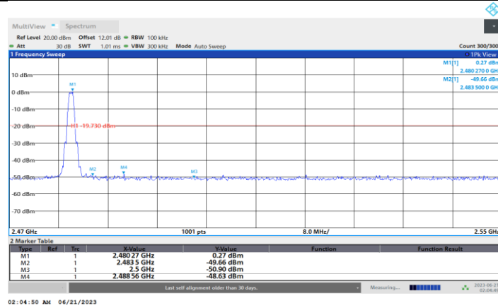
BLE_1M_Ant1_High_2480
