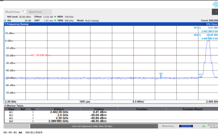
BLE_1M_Ant1_Low_2402
