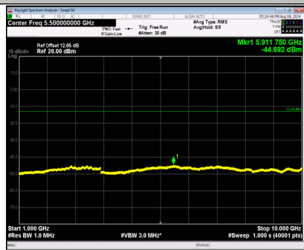
5-5-10MHz-10MHz-QPSK-QPSK-20450-20549-1RB#0-1 RB#49-1000~10000MHz-PASS
