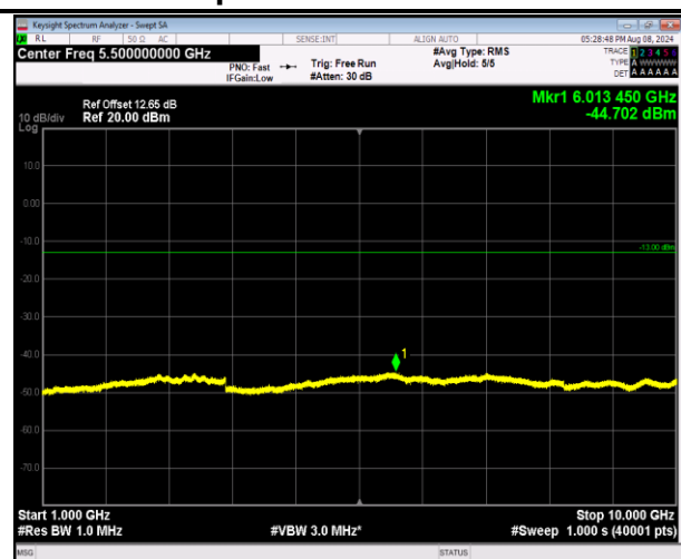
5-5-10MHz-10MHz-16QAM-16QAM-20476-20575-1RB#4 9-ORB#0-1000~10000MHz-PASS
