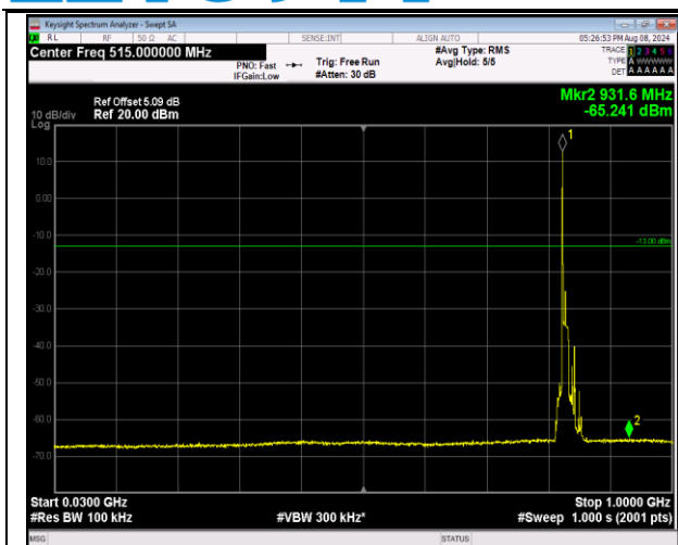
5-5-10MHz-10MHz-QPSK-QPSK-20476-20575-1RB#0-0 RB#0-30~1000MHz-PASS
