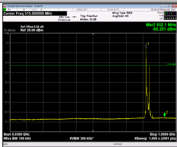
5-5-10MHz-10MHz-QPSK-QPSK-20450-20549-1RB#0-1 RB#49-30~1000MHz-PASS
