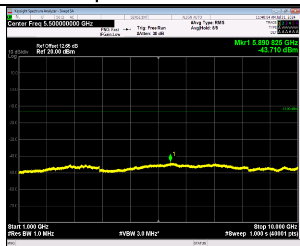
5-5-10MHz-10MHz-64QAM-64QAM-20476-20575-1RB#0 -1RB#49-1000~10000MHz-PASS
