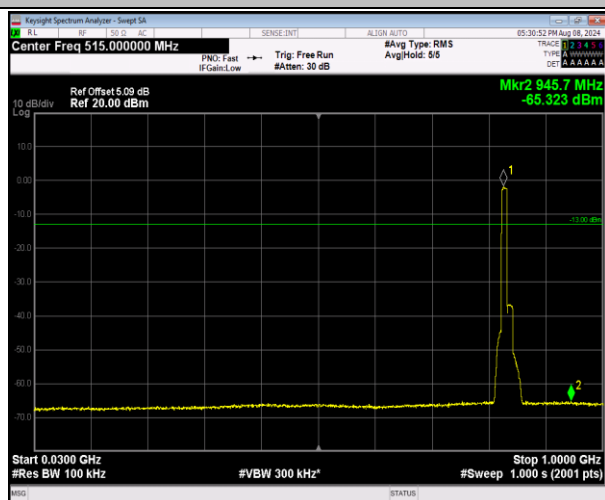
5-5-10MHz-10MHz-16QAM-16QAM-20476-20575-50RB #0-50RB#0-30~1000MHz-PASS
