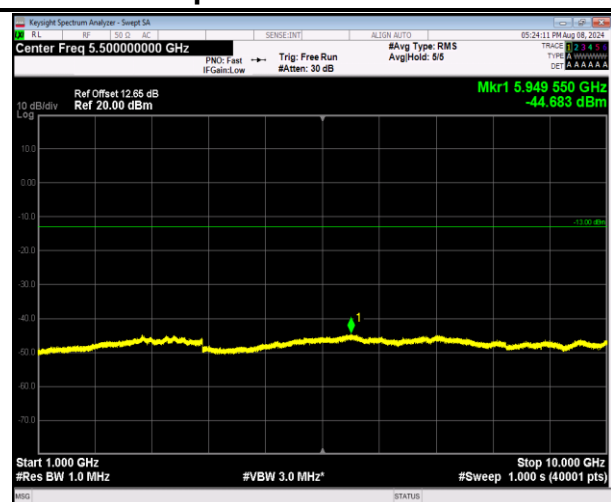
5-5-10MHz-10MHz-16QAM-16QAM-20450-20549-1RB#4 9-0RB#0-1000~10000MHz-PASS
