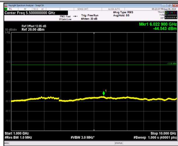
5-5-10MHz-10MHz-QPSK-QPSK-20450-20549-1RB#49-0 RB#0-1000~10000MHz-PASS
