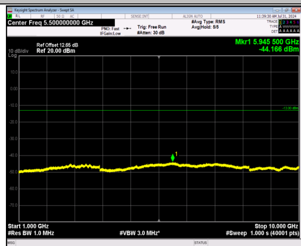
5-5-10MHz-10MHz-64QAM-64QAM-20476-20575-1RB#4 9-0RB#0-1000~10000MHz-PASS
