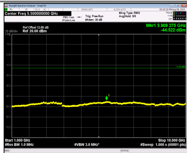
5-5-10MHz-10MHz-16QAM-16QAM-20450-20549-1RB#0-0-1RB#49-1000~10000MHz-PASS
