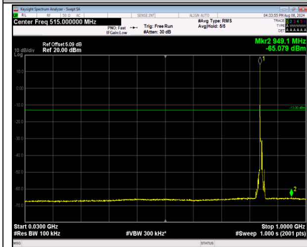
5-5-5MHz-3MHz-16QAM-16QAM-20595-20634-1RB#0-1 RB#15-30~1000MHz-PASS
