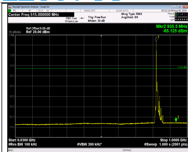
5-5-10MHz-10MHz-QPSK-QPSK-20450-20549-1RB#0-0 RB#0-30~1000MHz-PASS
