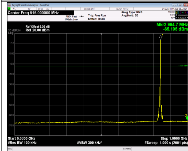
5-5-5MHz-3MHz-QPSK-QPSK-20595-20634-1RB#24-0R B#0-30~1000MHz-PASS
