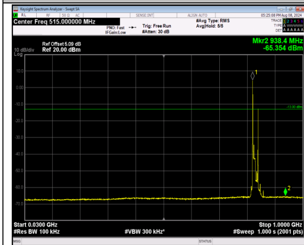
5-5-10MHz-10MHz-16QAM-16QAM-20450-20549-1RB#0-0-1RB#49-30~1000MHz-PASS
