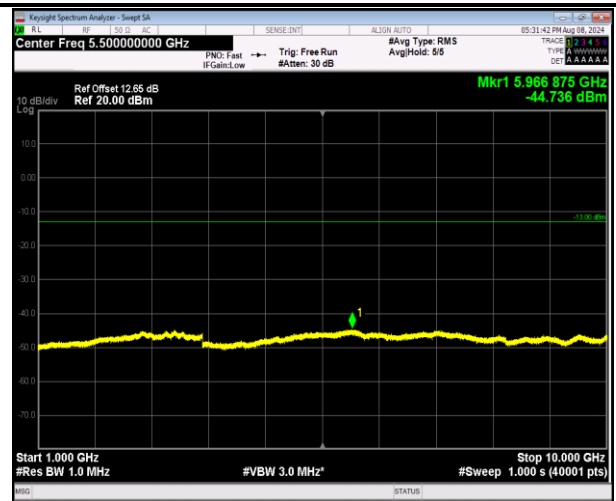
5-5-10MHz-10MHz-QPSK-QPSK-20501-20600-1RB#0-0 RB#0-1000~10000MHz-PASS
