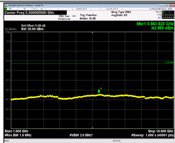
5-5-10MHz-10MHz-64QAM-64QAM-20476-20575-50RB# 0-50RB#0-1000~10000MHz-PASS
