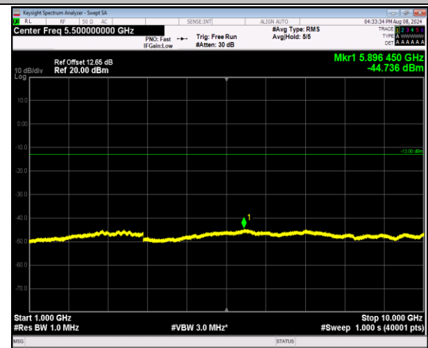
5-5-5MHz-3MHz-QPSK-QPSK-20595-20634-1RB#0-1RB #15-1000~10000MHz-PASS
