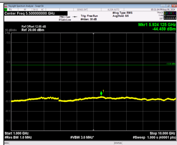
5-5-10MHz-10MHz-16QAM-16QAM-20476-20575-50RB# 0-50RB#0-1000~10000MHz-PASS
