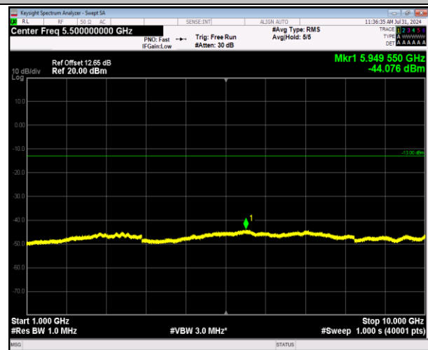
5-5-10MHz-10MHz-64QAM-64QAM-20450-20549-1RB#0 -0RB#0-1000~10000MHz-PASS
