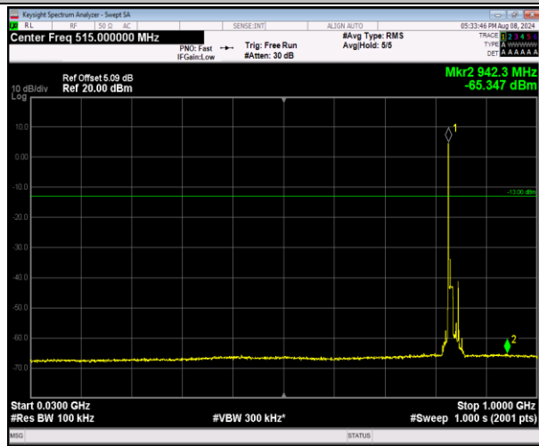
5-5-10MHz-10MHz-QPSK-QPSK-20501-20600-1RB#0-1 RB#49-30~1000MHz-PASS
