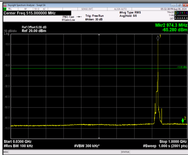
5-5-10MHz-10MHz-QPSK-QPSK-20501-20600-1RB#49-0 ORB#0-30~1000MHz-PASS
