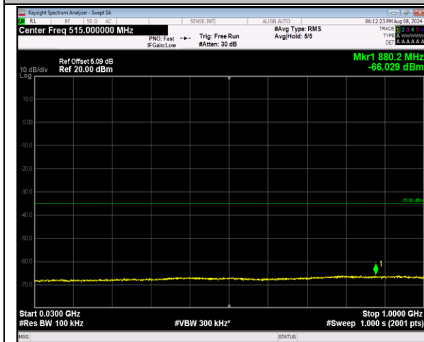
7-7-10MHz-20MHz-QPSK-QPSK-20805-20949-1RB#49- ORB#0-30~1000MHz-PASS
