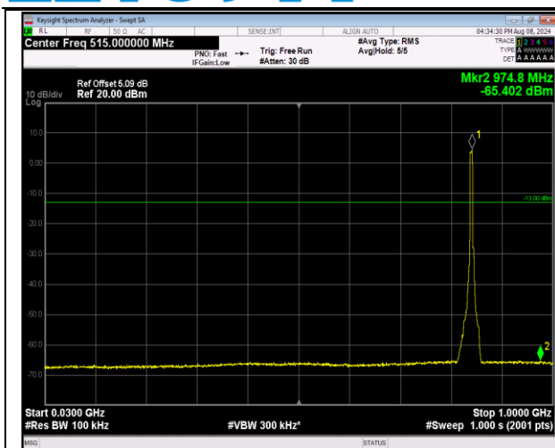
5-5-5MHz-3MHz-QPSK-QPSK-20595-20634-25RB#0-15 RB#0-30~1000MHz-PASS
