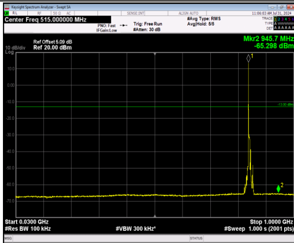
5-5-5MHz-3MHz-64QAM-64QAM-20595-20634-1RB#0-0RB#0-30~1000MHz-PASS
