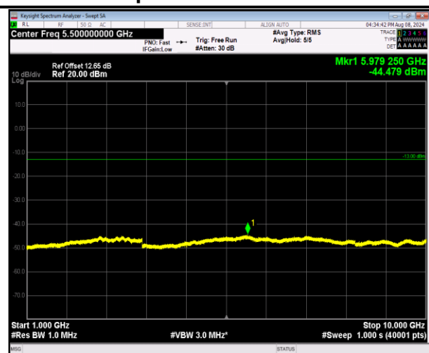
5-5-5MHz-3MHz-QPSK-QPSK-20595-20634-25RB#0-15 RB#0-1000~10000MHz-PASS
