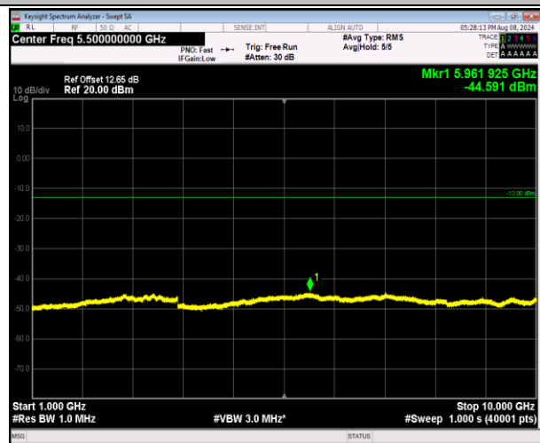
5-5-10MHz-10MHz-QPSK-QPSK-20476-20575-1RB#49-0 RB#0-1000~10000MHz-PASS
