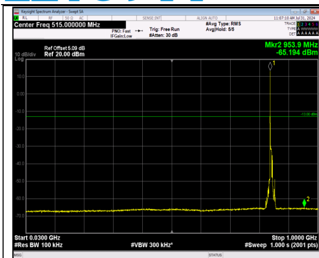
5-5-5MHz-3MHz-64QAM-64QAM-20595-20634-1RB#0-1 RB#15-30~1000MHz-PASS
