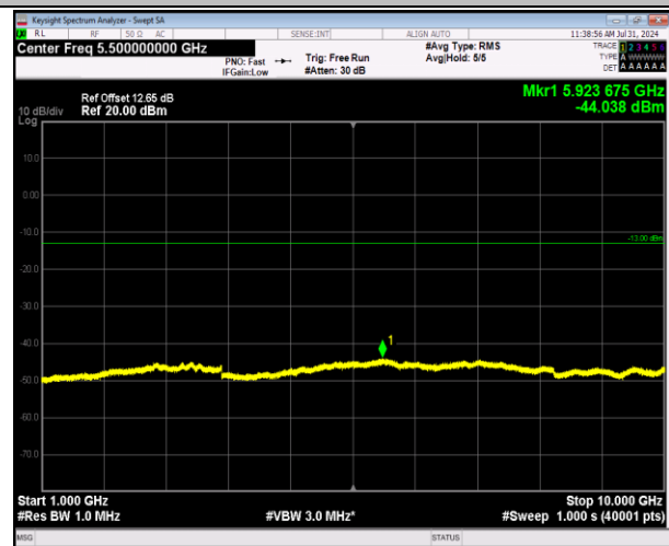
5-5-10MHz-10MHz-64QAM-64QAM-20476-20575-1RB#0 -ORB#0-1000~10000MHz-PASS
