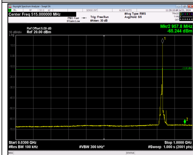
5-5-10MHz-10MHz-64QAM-64QAM-20476-20575-1RB# 49-0RB#0-30~1000MHz-PASS
