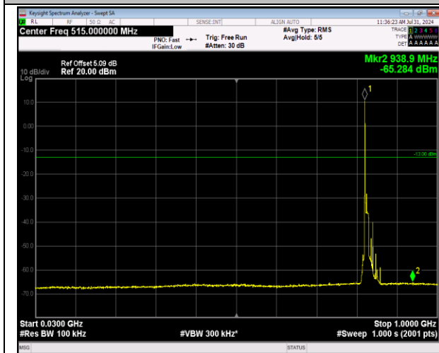
5-5-10MHz-10MHz-64QAM-64QAM-20450-20549-1RB# 0-0RB#0-30~1000MHz-PASS
