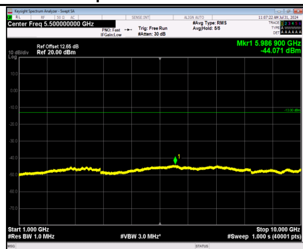
5-5-5MHz-3MHz-64QAM-64QAM-20595-20634-1RB#0-1 RB#15-1000~10000MHz-PASS
