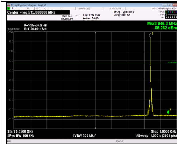
5-5-5MHz-3MHz-QPSK-QPSK-20595-20634-1RB#0-0R B#0-30~1000MHz-PASS
