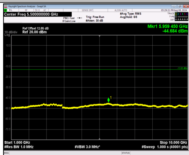
5-5-10MHz-10MHz-QPSK-QPSK-20476-20575-1RB#0-1 RB#49-1000~10000MHz-PASS
