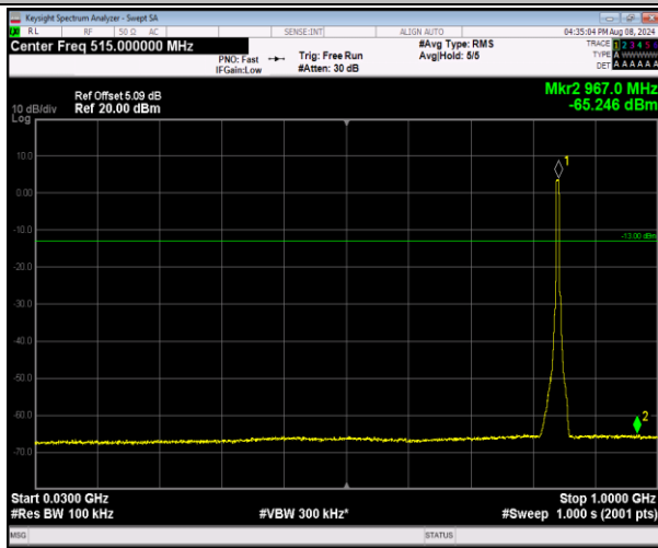
5-5-5MHz-3MHz-16QAM-16QAM-20595-20634-25RB#0-15RB#0-30~1000MHz-PASS
