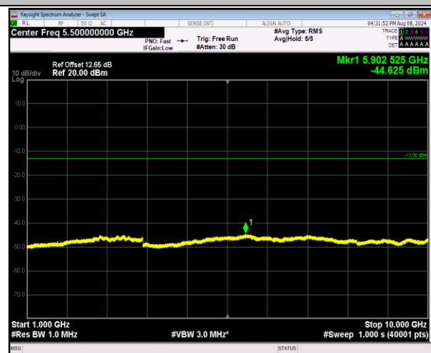
5-5-5MHz-3MHz-16QAM-16QAM-20595-20634-1RB#0-0 RB#0-1000~10000MHz-PASS
