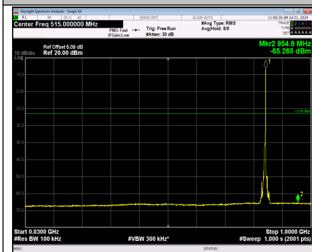
5-5-5MHz-3MHz-64QAM-64QAM-20595-20634-1RB#24- ORB#0-30~1000MHz-PASS
