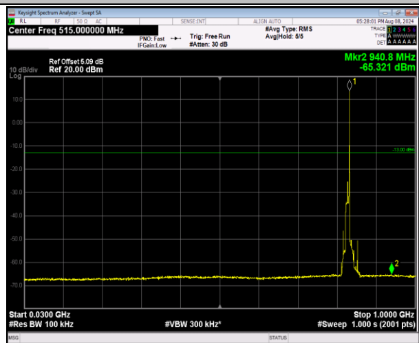
5-5-10MHz-10MHz-QPSK-QPSK-20476-20575-1RB#49- ORB#0-30~1000MHz-PASS
