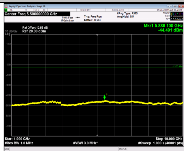
5-5-10MHz-10MHz-16QAM-16QAM-20450-20549-50RB# 0-50RB#0-1000~10000MHz-PASS
