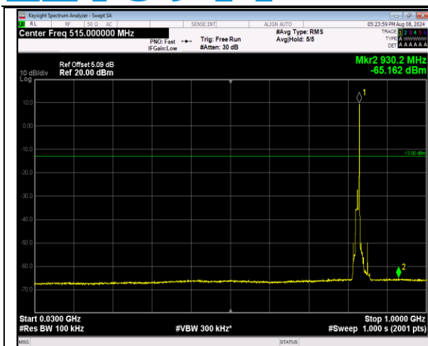
5-5-10MHz-10MHz-16QAM-16QAM-20450-20549-1RB# 49-0RB#0-30~1000MHz-PASS
