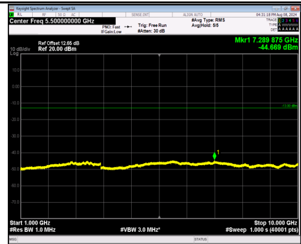
5-5-5MHz-3MHz-QPSK-QPSK-20595-20634-1RB#0-0RB #0-1000~10000MHz-PASS
