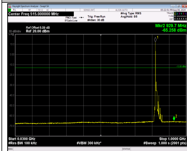
5-5-10MHz-10MHz-16QAM-16QAM-20450-20549-1RB#0-0RB#0-30~1000MHz-PASS
