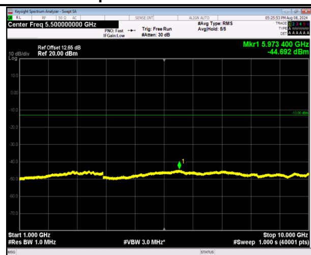
5-5-10MHz-10MHz-QPSK-QPSK-20450-20549-50RB#0-50RB#0-1000~10000MHz-PASS
