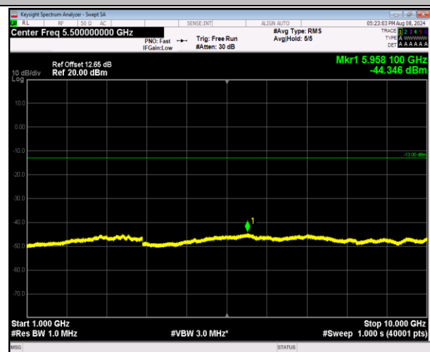
5-5-10MHz-10MHz-16QAM-16QAM-20450-20549-1RB#0-0RB#0-1000~10000MHz-PASS
