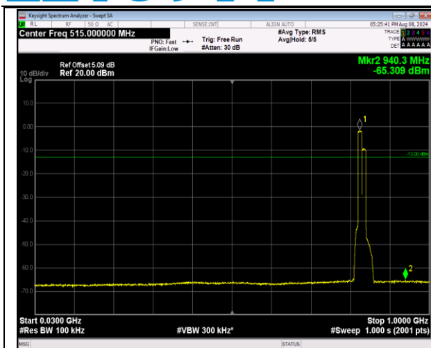
5-5-10MHz-10MHz-QPSK-QPSK-20450-20549-50RB#0-50RB#0-30~1000MHz-PASS
