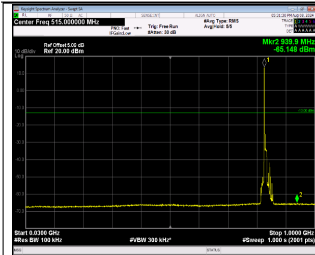
5-5-10MHz-10MHz-QPSK-QPSK-20501-20600-1RB#0-0 RB#0-30~1000MHz-PASS
