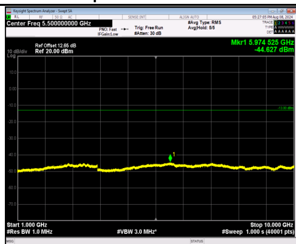
5-5-10MHz-10MHz-QPSK-QPSK-20476-20575-1RB#0-0 RB#0-1000~10000MHz-PASS
