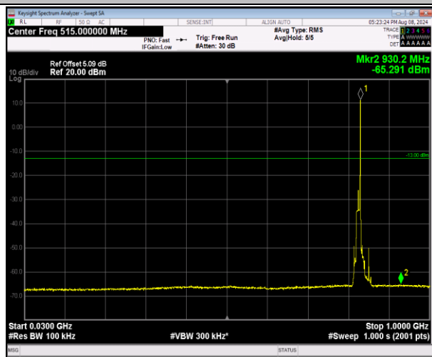
5-5-10MHz-10MHz-QPSK-QPSK-20450-20549-1RB#49-0 ORB#0-30~1000MHz-PASS
