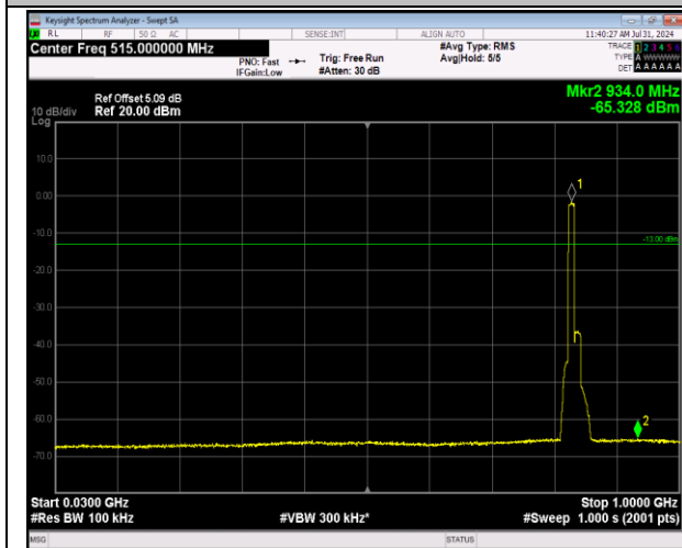
5-5-10MHz-10MHz-64QAM-64QAM-20476-20575-50RB #0-50RB#0-30~1000MHz-PASS
