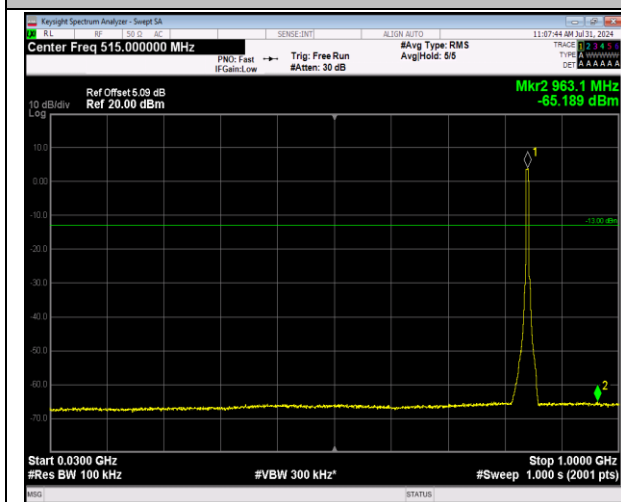
5-5-5MHz-3MHz-64QAM-64QAM-20595-20634-25RB#0- 15RB#0-30~1000MHz-PASS
