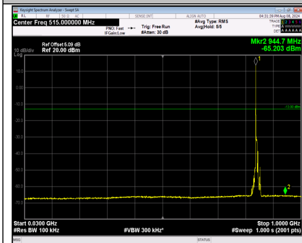
5-5-5MHz-3MHz-16QAM-16QAM-20595-20634-1RB#0-0 RB#0-30~1000MHz-PASS
