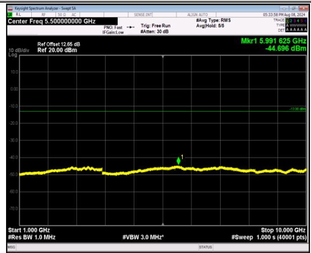
5-5-10MHz-10MHz-QPSK-QPSK-20501-20600-1RB#0-1 RB#49-1000~10000MHz-PASS
