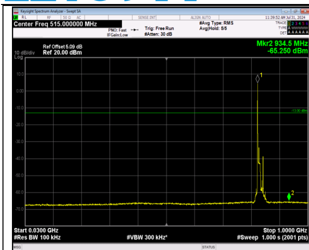
5-5-10MHz-10MHz-64QAM-64QAM-20476-20575-1RB# 0-1RB#49-30~1000MHz-PASS
