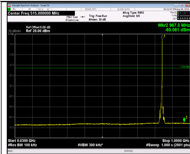
5-5-5MHz-3MHz-16QAM-16QAM-20595-20634-1RB#24-ORB#0-30~1000MHz-PASS
