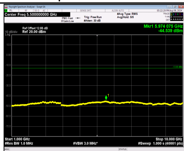
5-5-10MHz-10MHz-QPSK-QPSK-20450-20549-1RB#0-0 RB#0-1000~10000MHz-PASS
