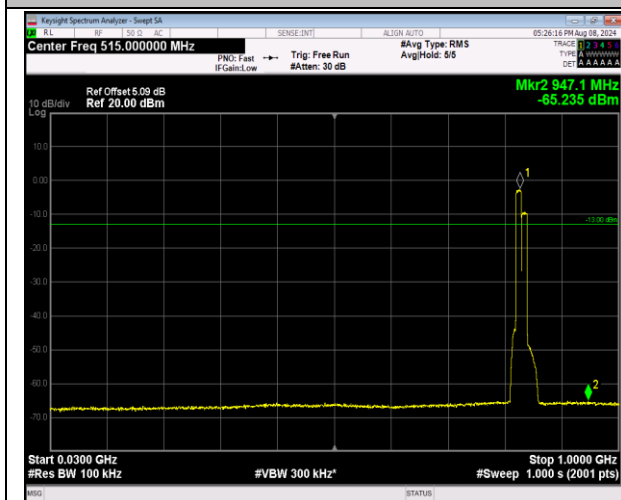
5-5-10MHz-10MHz-16QAM-16QAM-20450-20549-50RB #0-50RB#0-30~1000MHz-PASS
