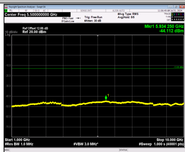
5-5-5MHz-3MHz-64QAM-64QAM-20595-20634-1RB#24- ORB#0-1000~10000MHz-PASS
