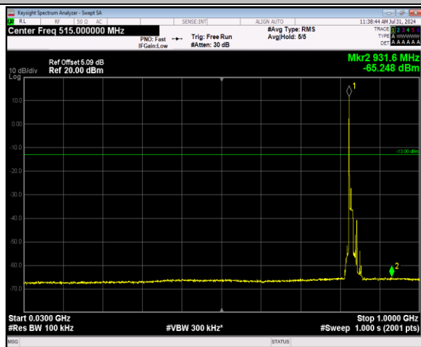
5-5-10MHz-10MHz-64QAM-64QAM-20476-20575-1RB# 0-ORB#0-30~1000MHz-PASS
