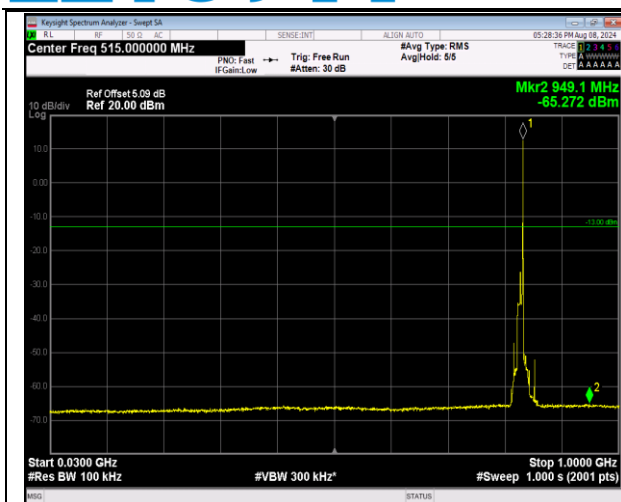
5-5-10MHz-10MHz-16QAM-16QAM-20476-20575-1RB# 49-ORB#0-30~1000MHz-PASS
