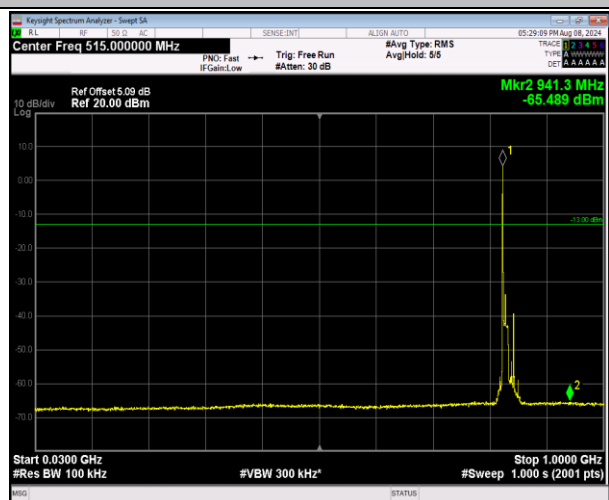
5-5-10MHz-10MHz-QPSK-QPSK-20476-20575-1RB#0-1 RB#49-30~1000MHz-PASS
