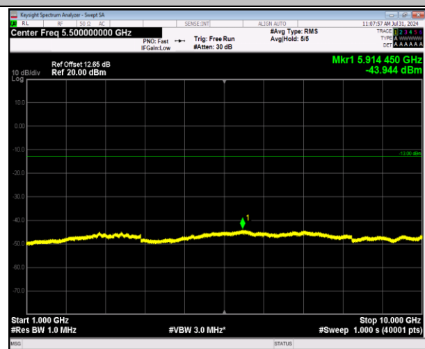
5-5-5MHz-3MHz-64QAM-64QAM-20595-20634-25RB#0- 15RB#0-1000~10000MHz-PASS
