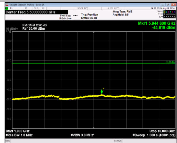
5-5-5MHz-3MHz-QPSK-QPSK-20595-20634-1RB#24-0R B#0-1000~10000MHz-PASS
