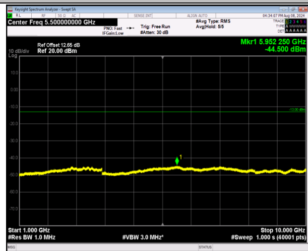
5-5-5MHz-3MHz-16QAM-16QAM-20595-20634-1RB#0-1 RB#15-1000~10000MHz-PASS
