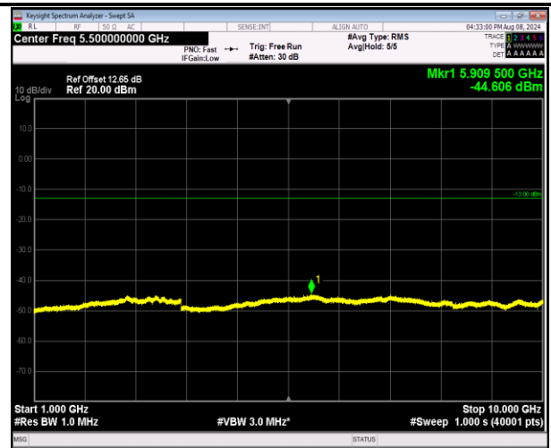
5-5-5MHz-3MHz-16QAM-16QAM-20595-20634-1RB#24-ORB#0-1000~10000MHz-PASS
